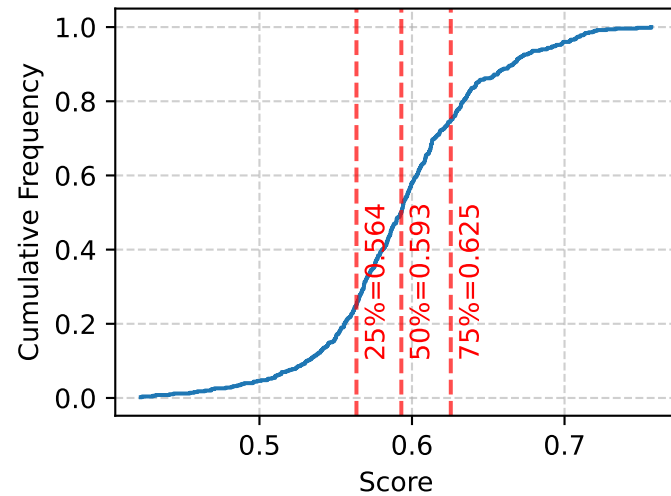
Entropy - BGE
