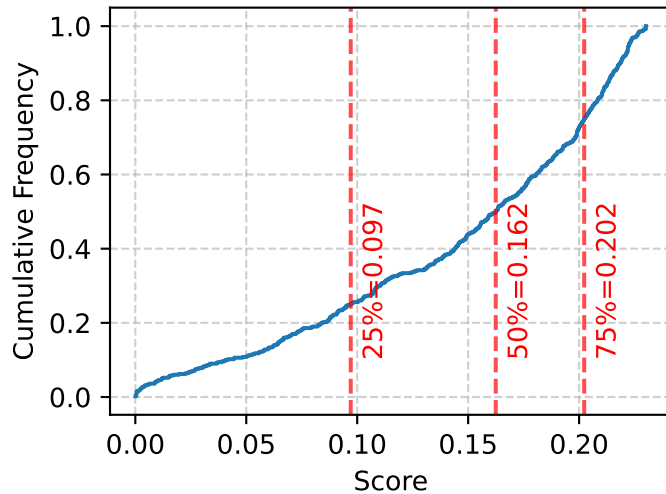
Entropy - MPNet
