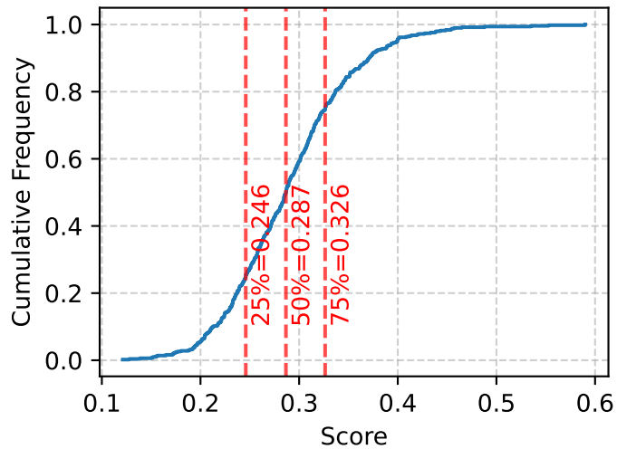
Entropy - MPNet
