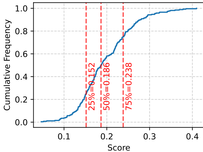
Entropy - MPNet
