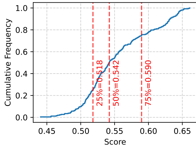
Entropy - BGE
