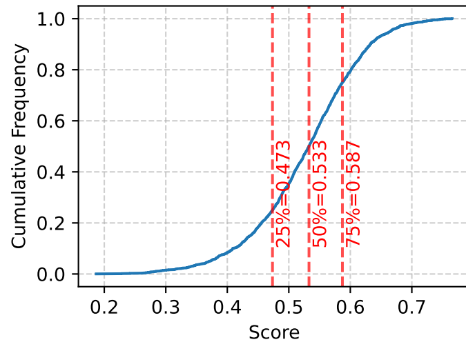
Entropy - 1M
