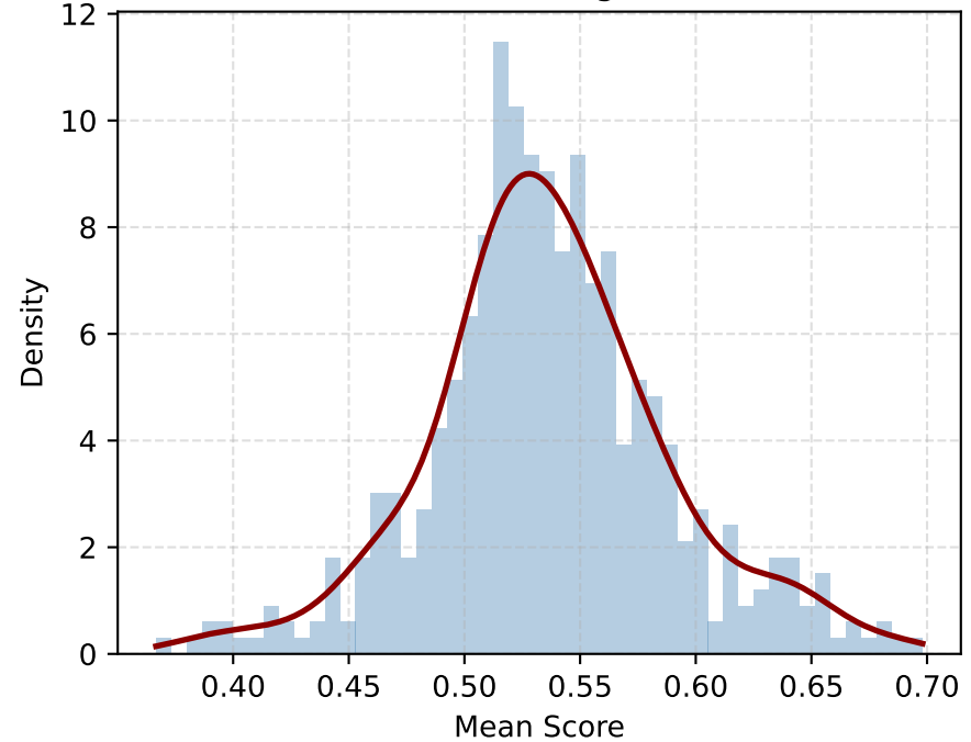
BGE - Histogram
