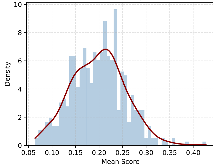
MiniLM - Histogram
