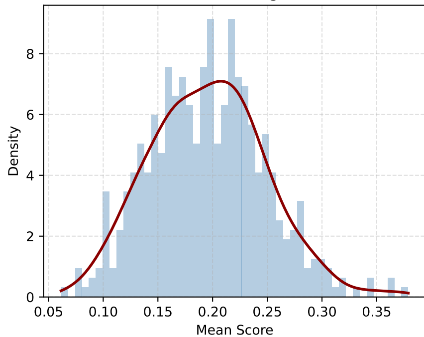
MPNet - Histogram
