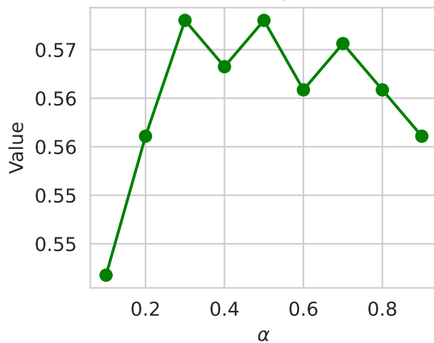
Recall@10
