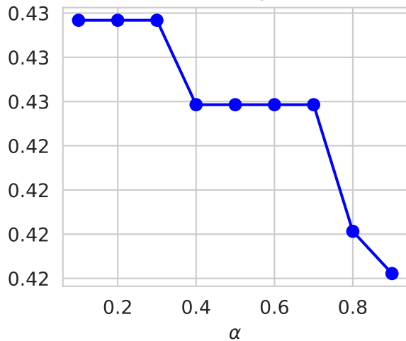
Recall@5
