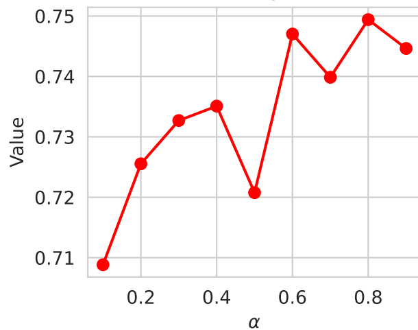
Recall@50
