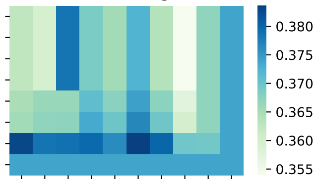
BGE (Recall@10)
