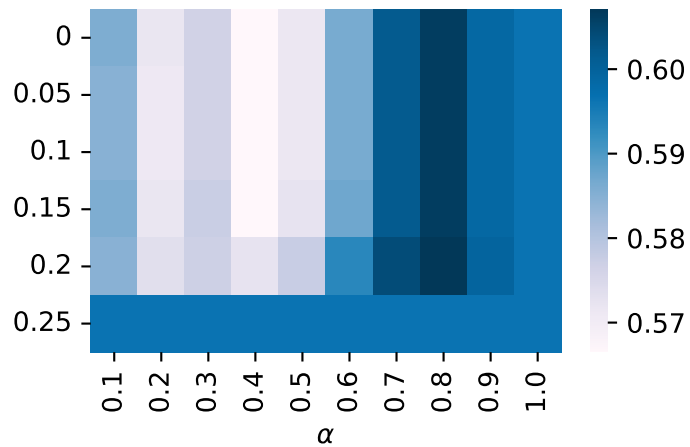
MiniLM (Recall@10)
