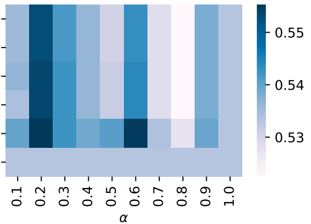
MPNet (Recall@10)
