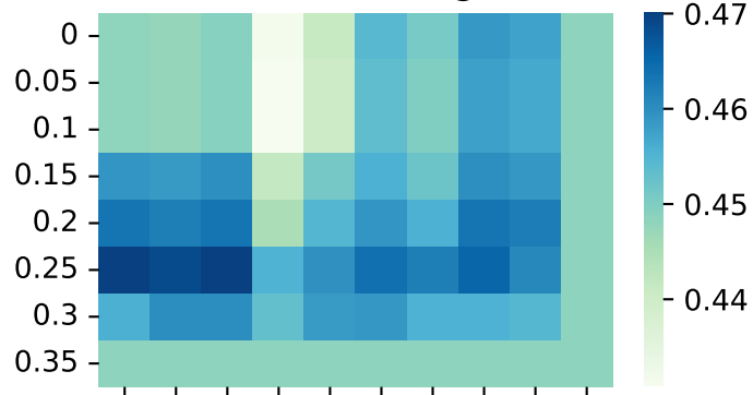
MiniLM (Recall@10)
