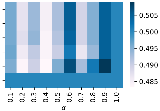
BGE (Recall@10)
