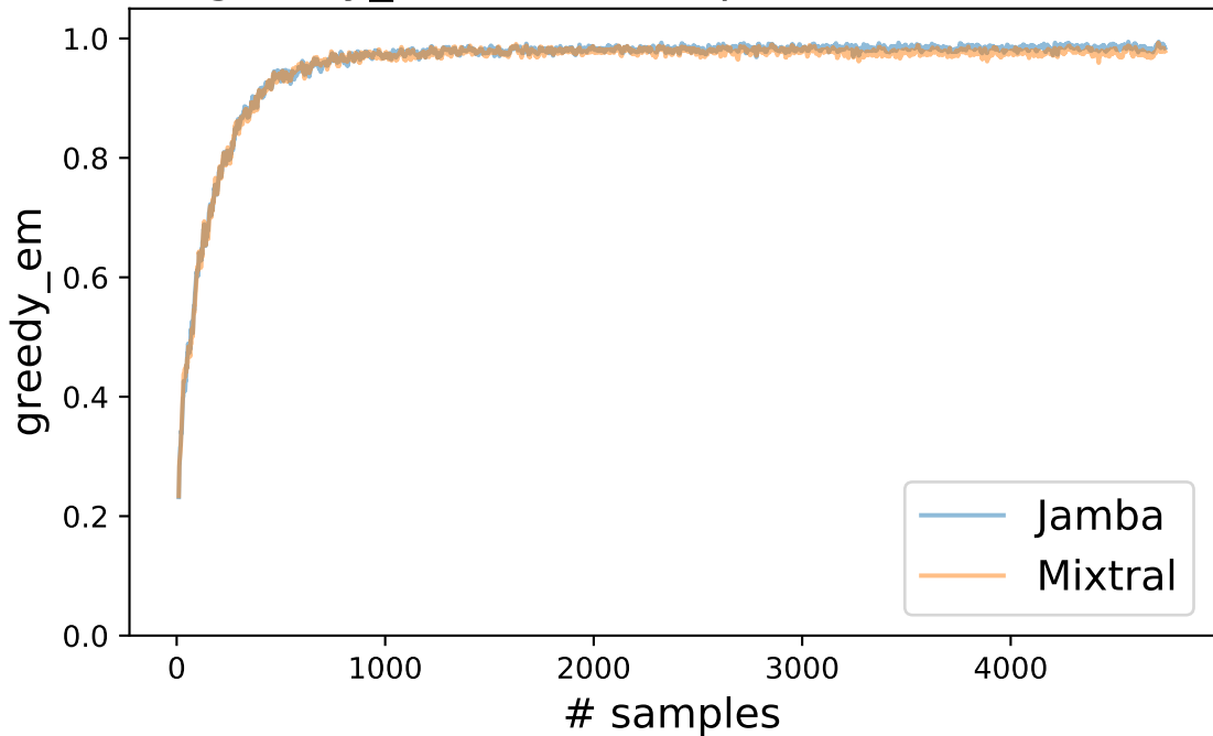
greedy_em vs. # samples for CLINC150
