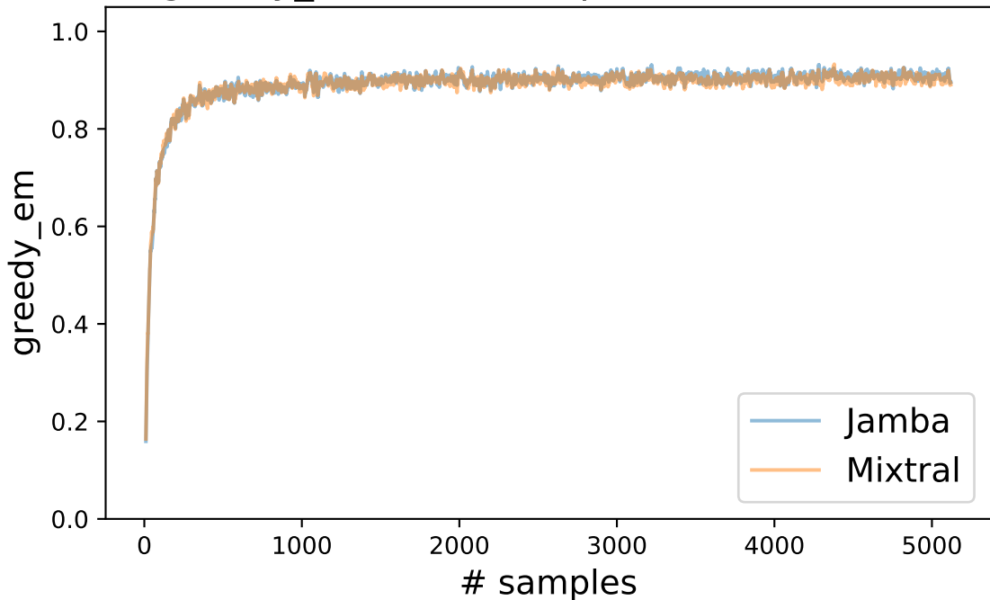
greedy_em vs. # samples for NLU Intent
