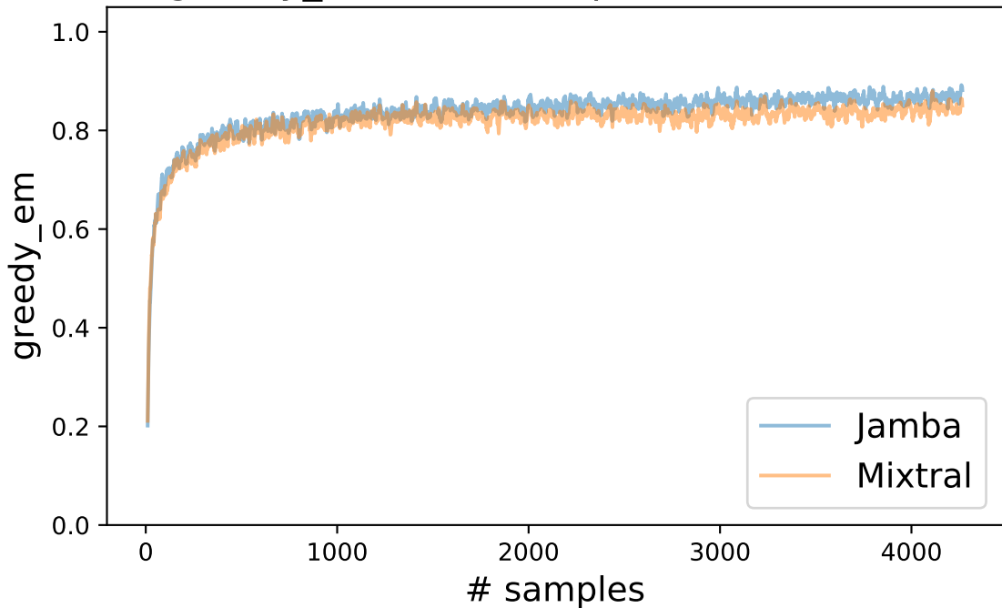
greedy_em vs. # samples for TREC-Fine
