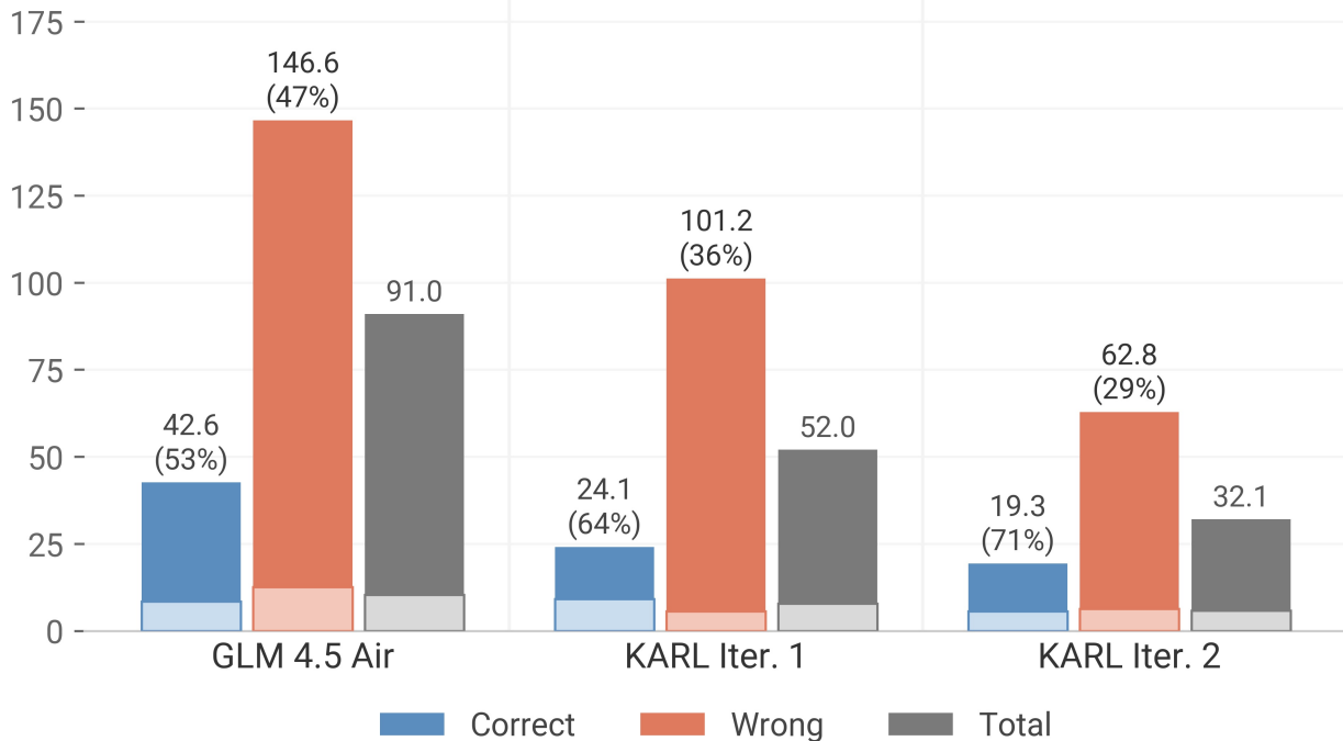
Search Efficiency on Common Perfect-Recall BrowseComp-Plus Instances (n=87)
