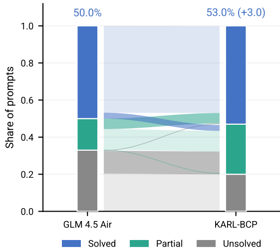
Pass Rate Flow
