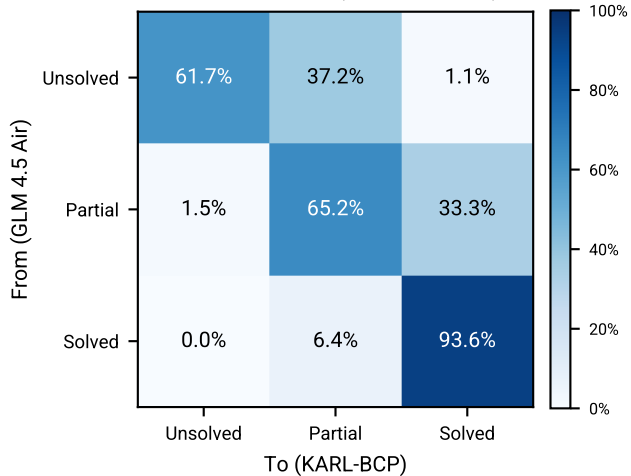
Transition Matrix (row-normalized)
