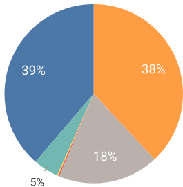
GLM 4.5 Air
