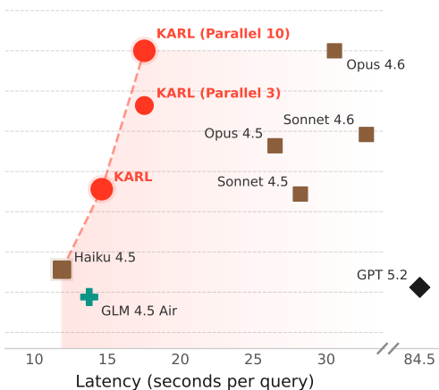
Latency-Quality Pareto
