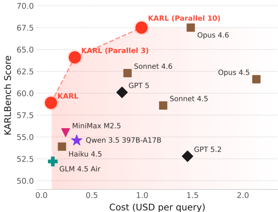
Cost-Quality Pareto
