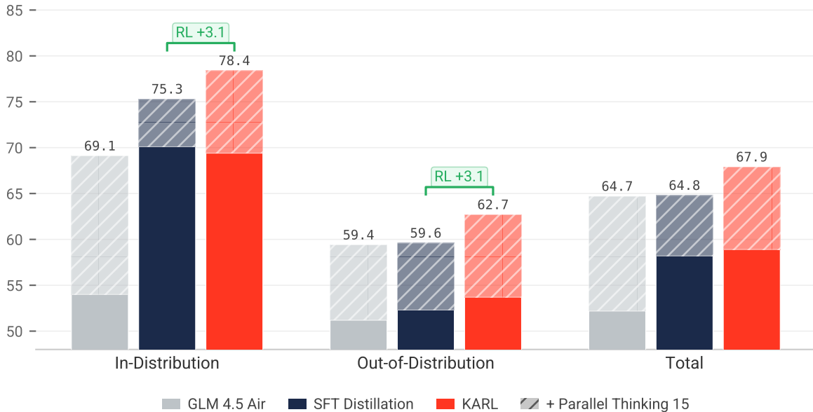
Average Score
