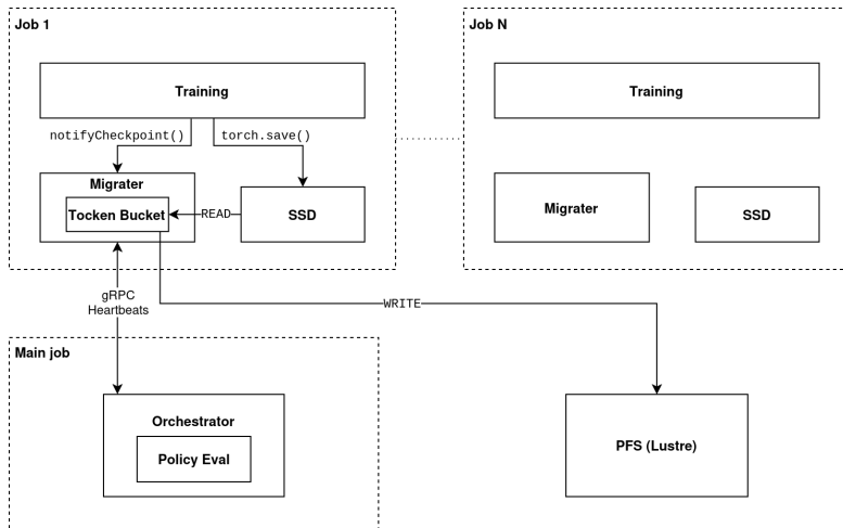
Figure 1. System Architecture.
