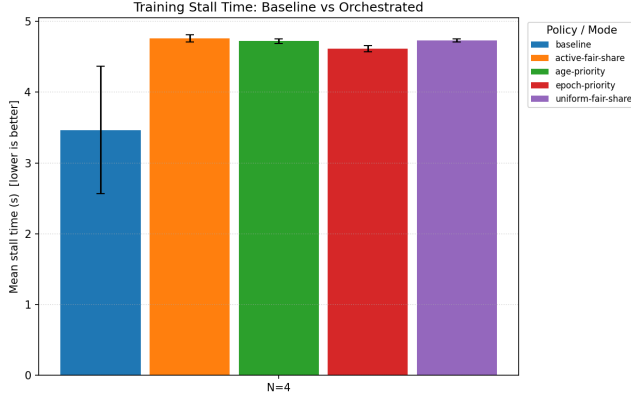
Figure 2. Comparison of stall durations during checkpointing. Tests were conducted on Deucalion with synthetic a checkpoint workload, saving checkpoints with 5GB size, as mentioned in the Benchmarks section.
