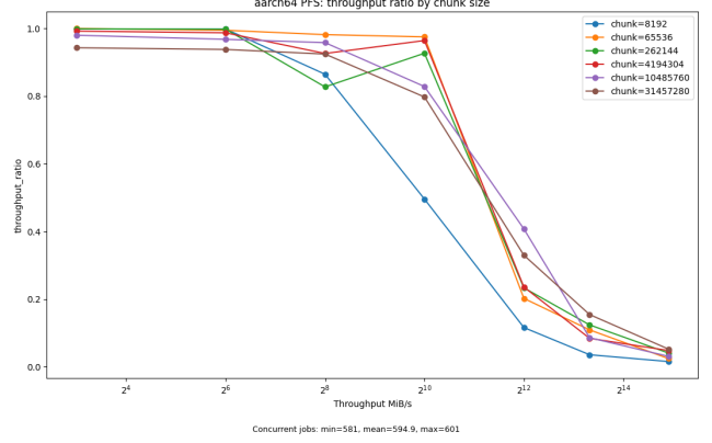
Figure 5. Token bucket actual/expected throughput ratio on the PFS for different chunk sizes and configured throughput targets. The 4 MiB chunk size provides a practical balance between throughput accuracy and reduced write frequency.
