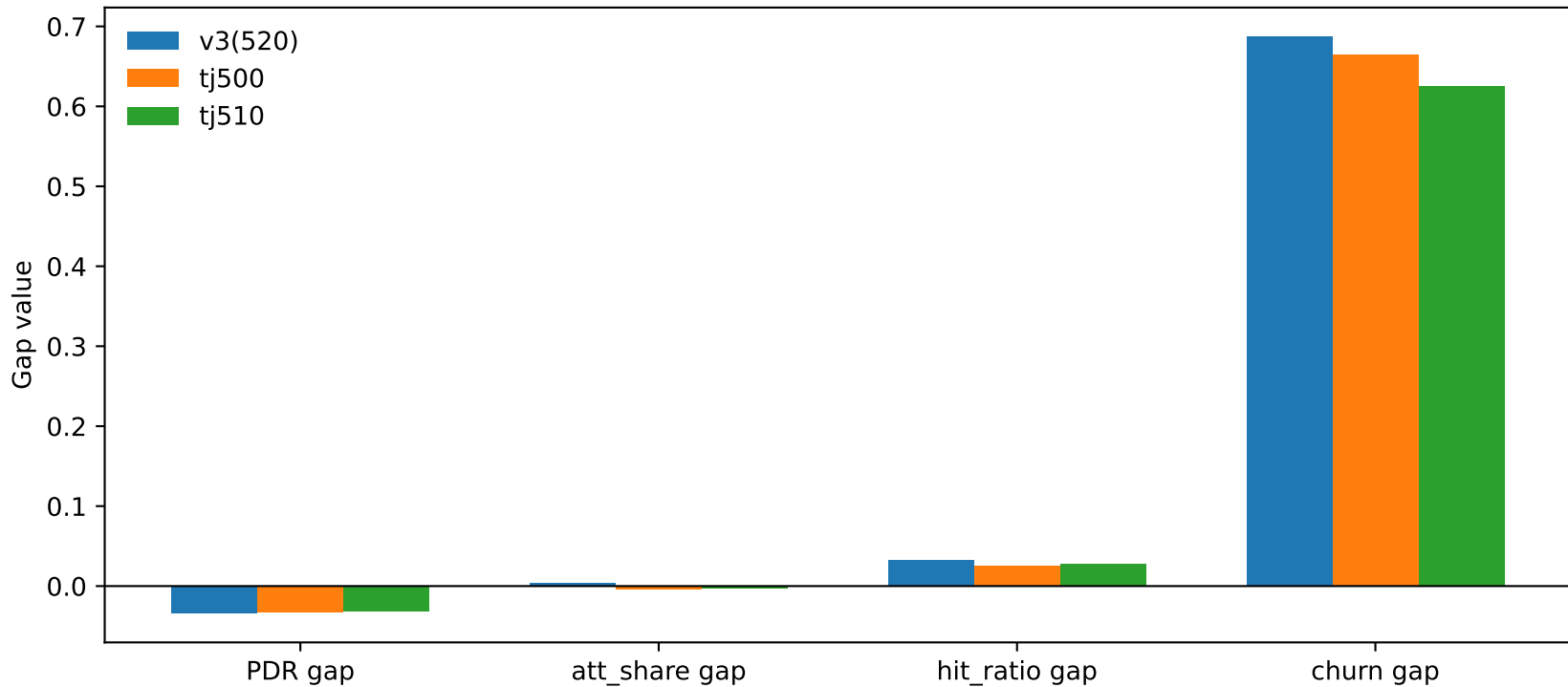
Mean Gap (TA-BRPL - BRPL)
