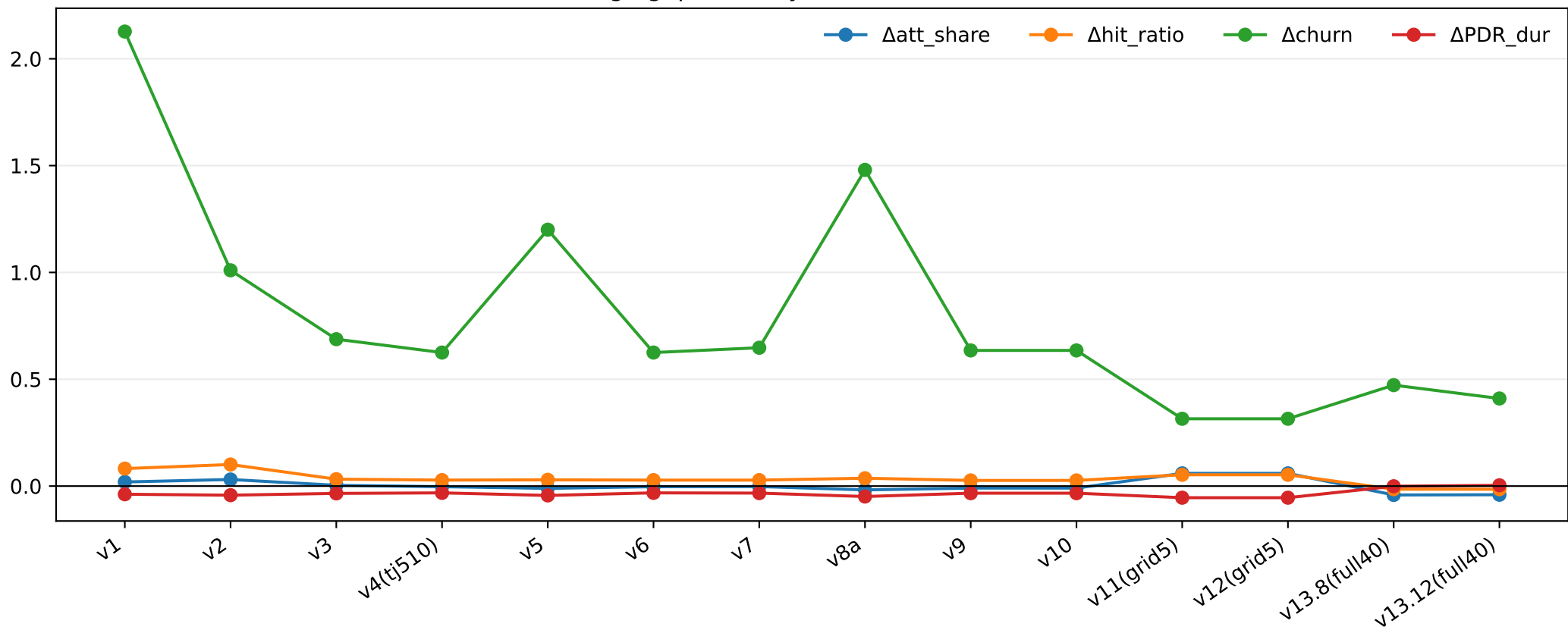
Average gap trend by version (v1 -&gt; v13.12)
