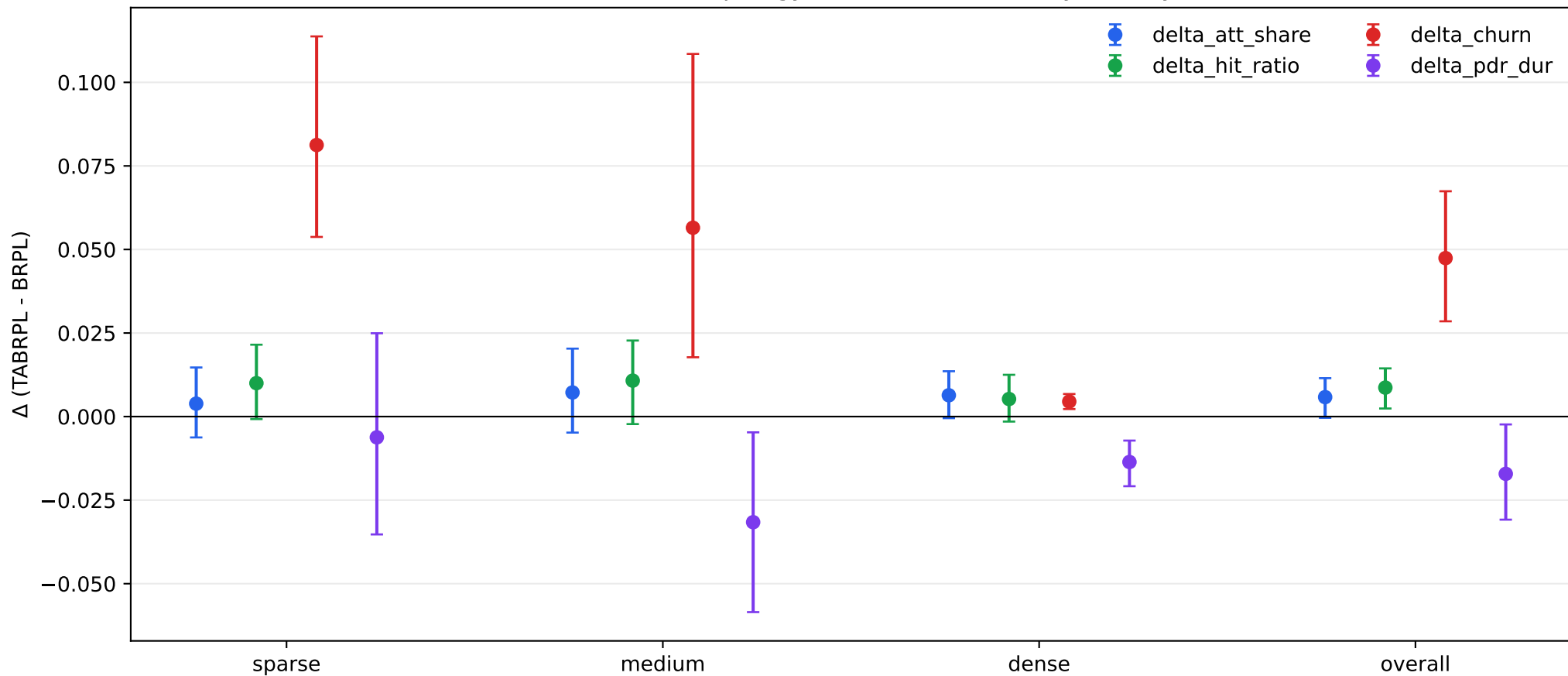
Main random-topology: delta with 95% CI by density
