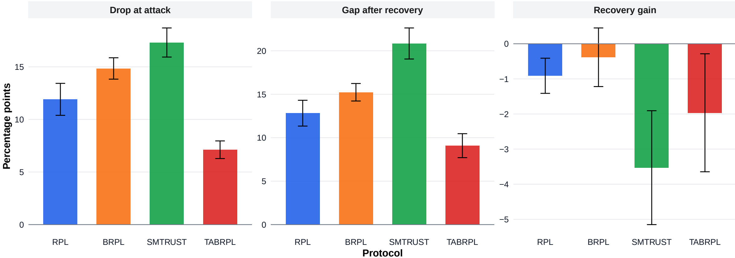
Fig. 2. Attack Damage and Recovery by Protocol
