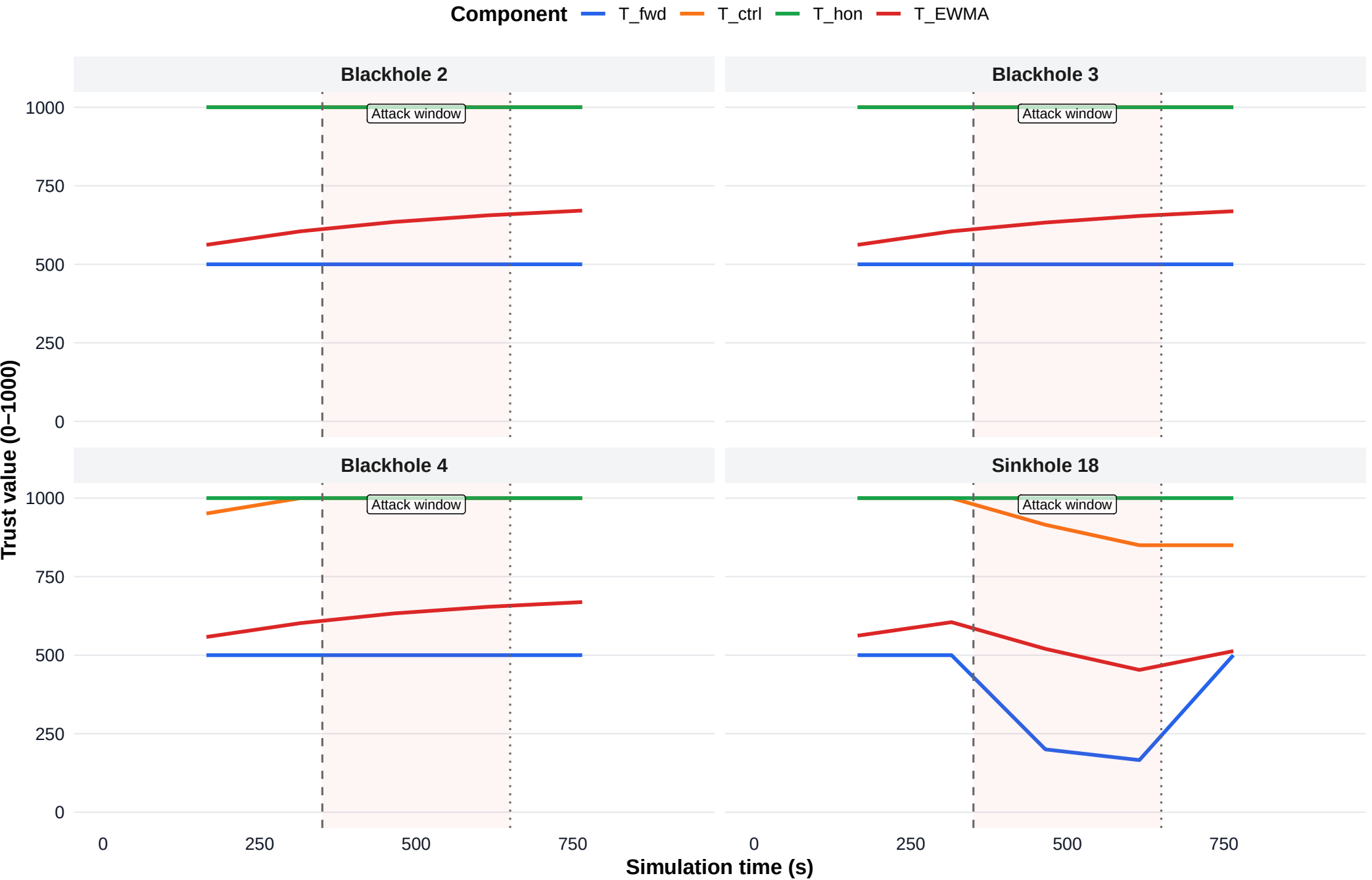
Fig. 5. TABRPL Trust Dynamics for Adversarial Neighbors Each panel shows the median component trajectory for one adversarial neighbor.
