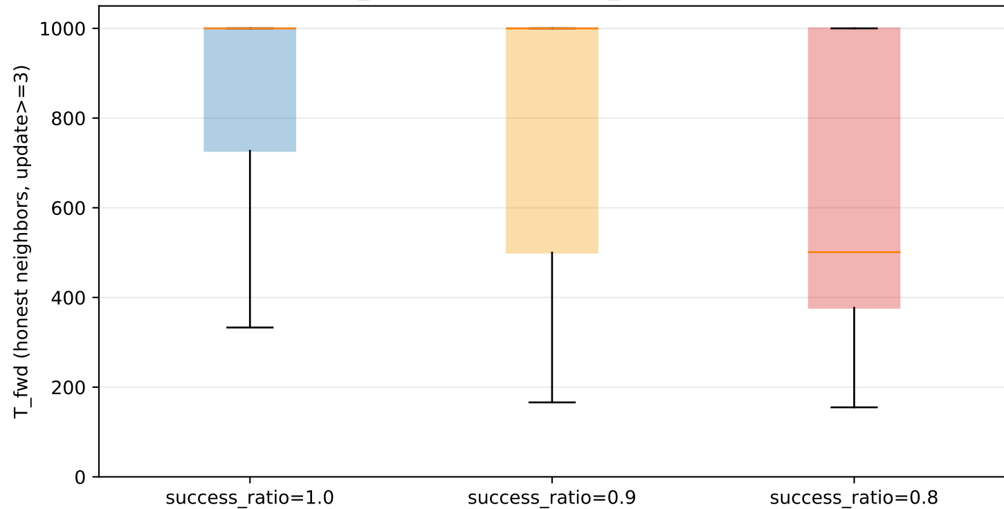
fig_loss: Link Loss vs T_fwd Collapse
