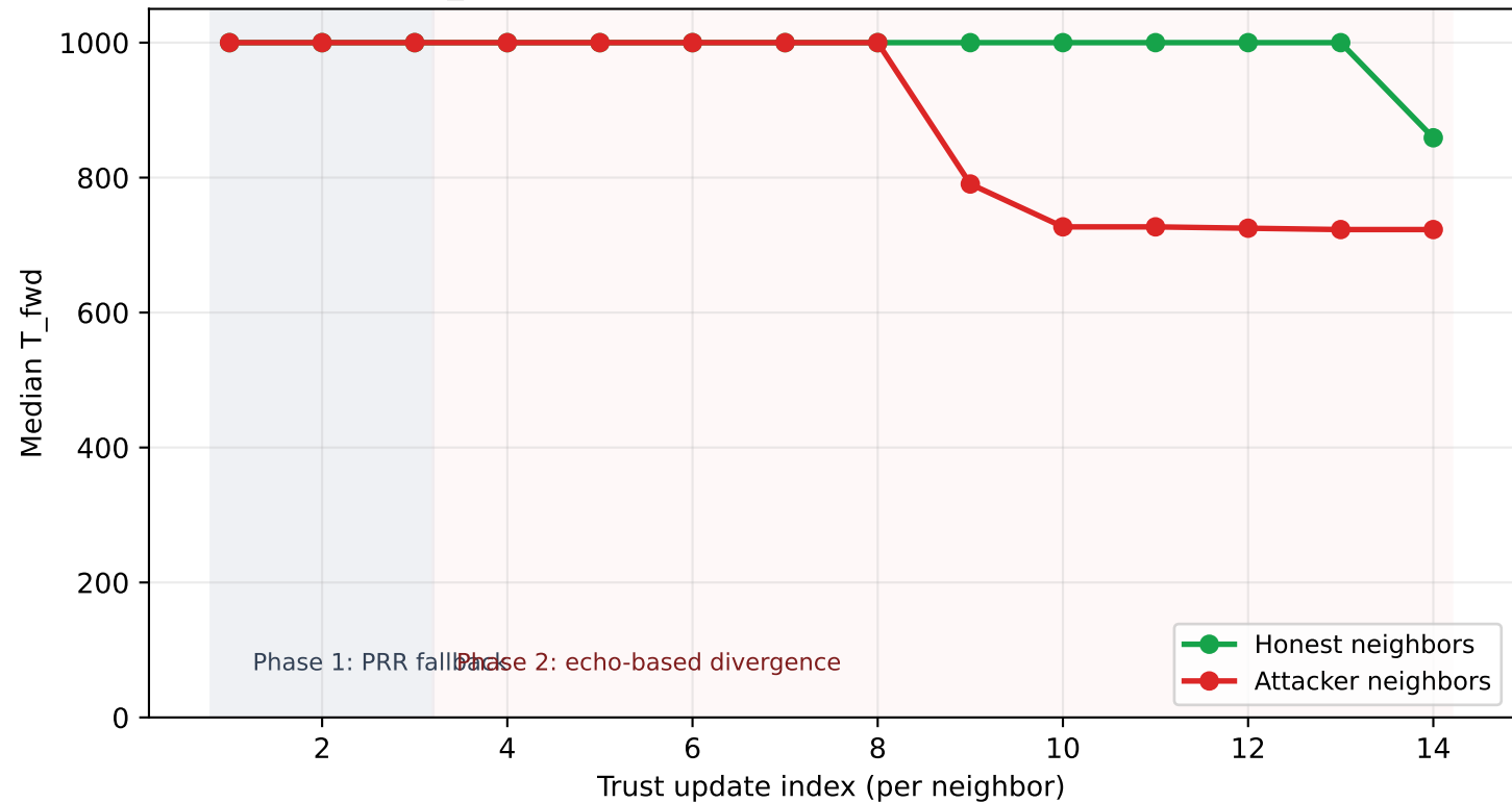
fig_twophase: Two-Phase Detection Trajectory
