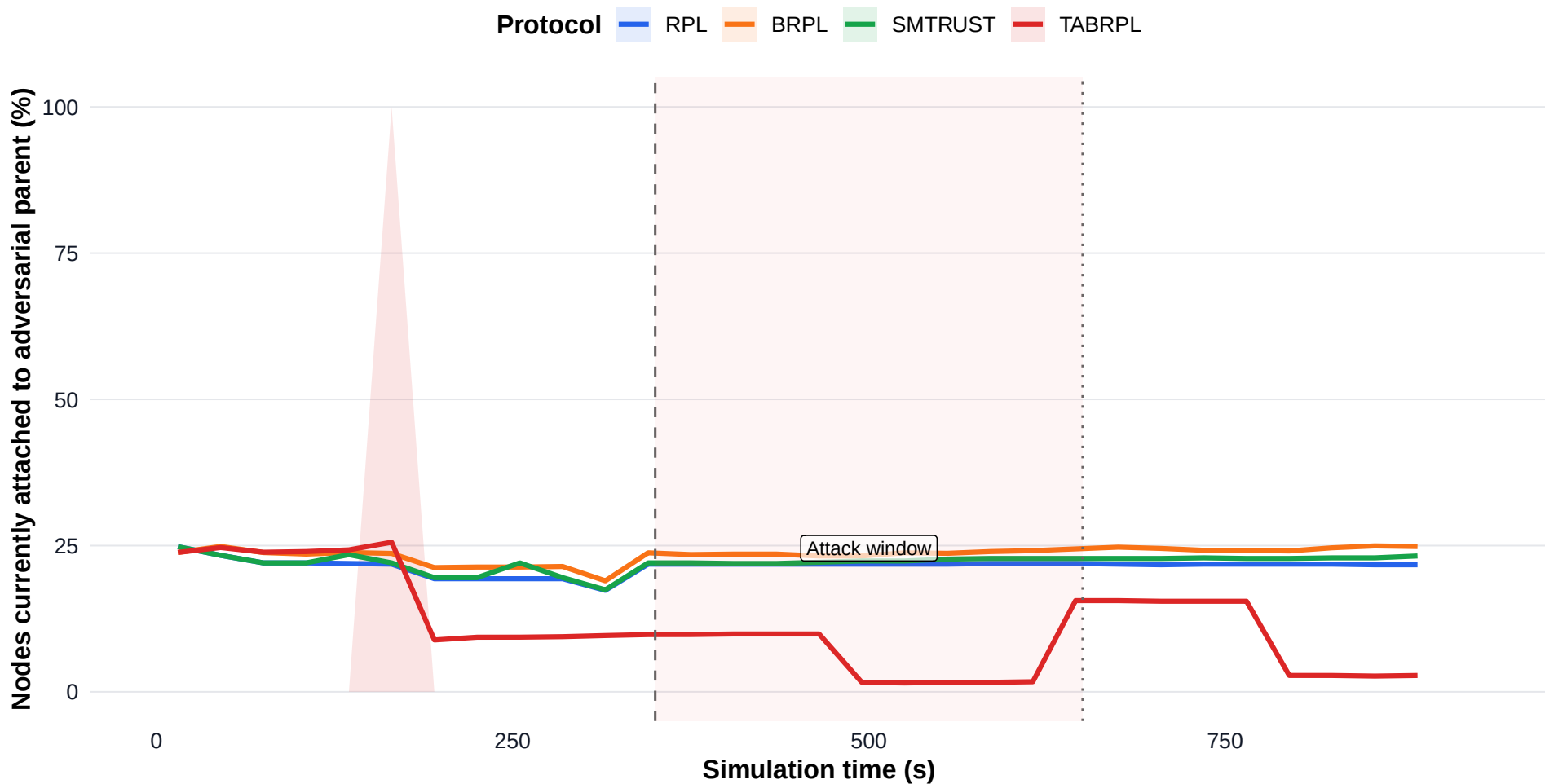
Fig. 4. Exposure to Adversarial Parents Over Time
