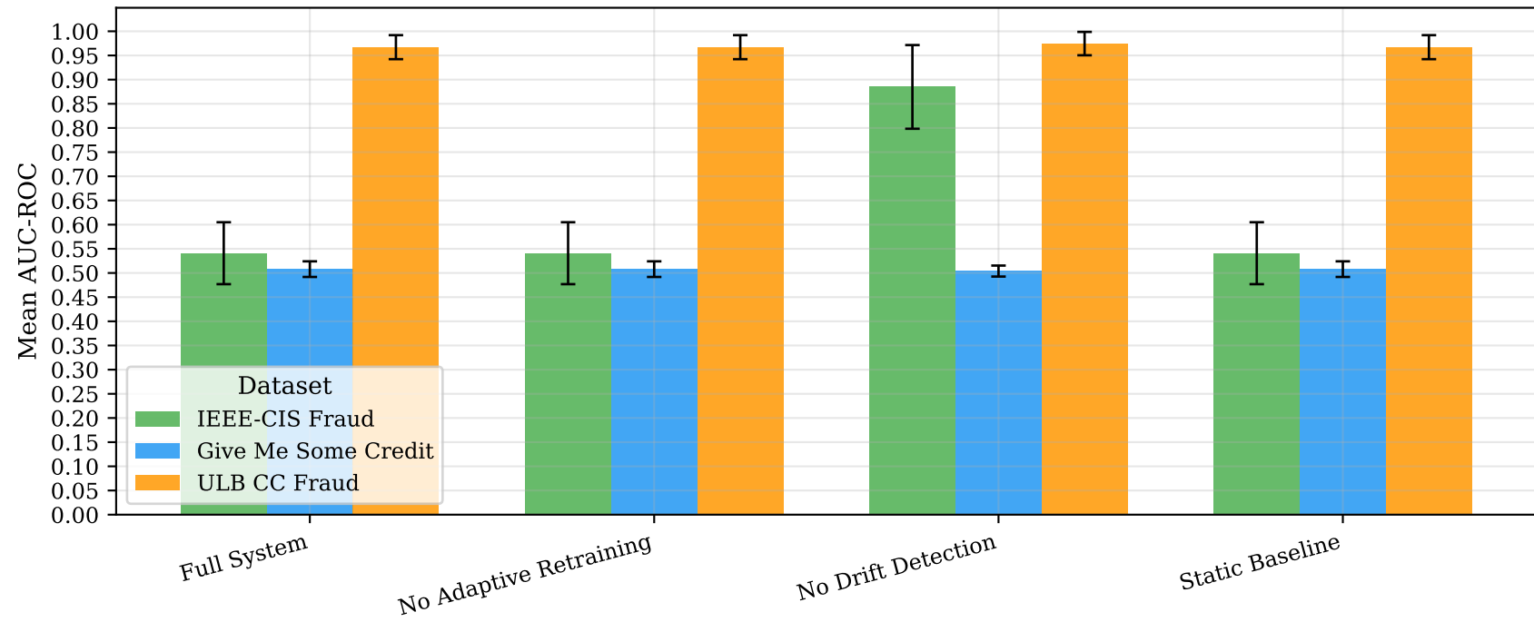
Ablation Study: Component Contribution to Performance
