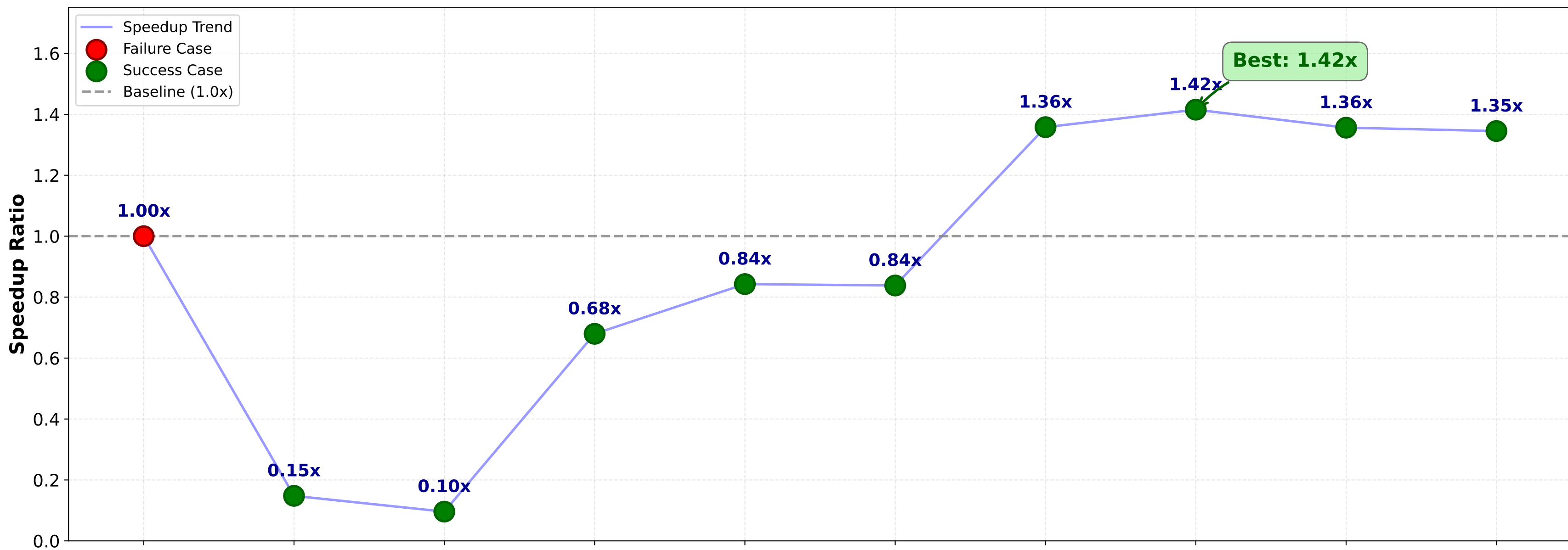
(b) LayerNorm2D Optimization in MNN
