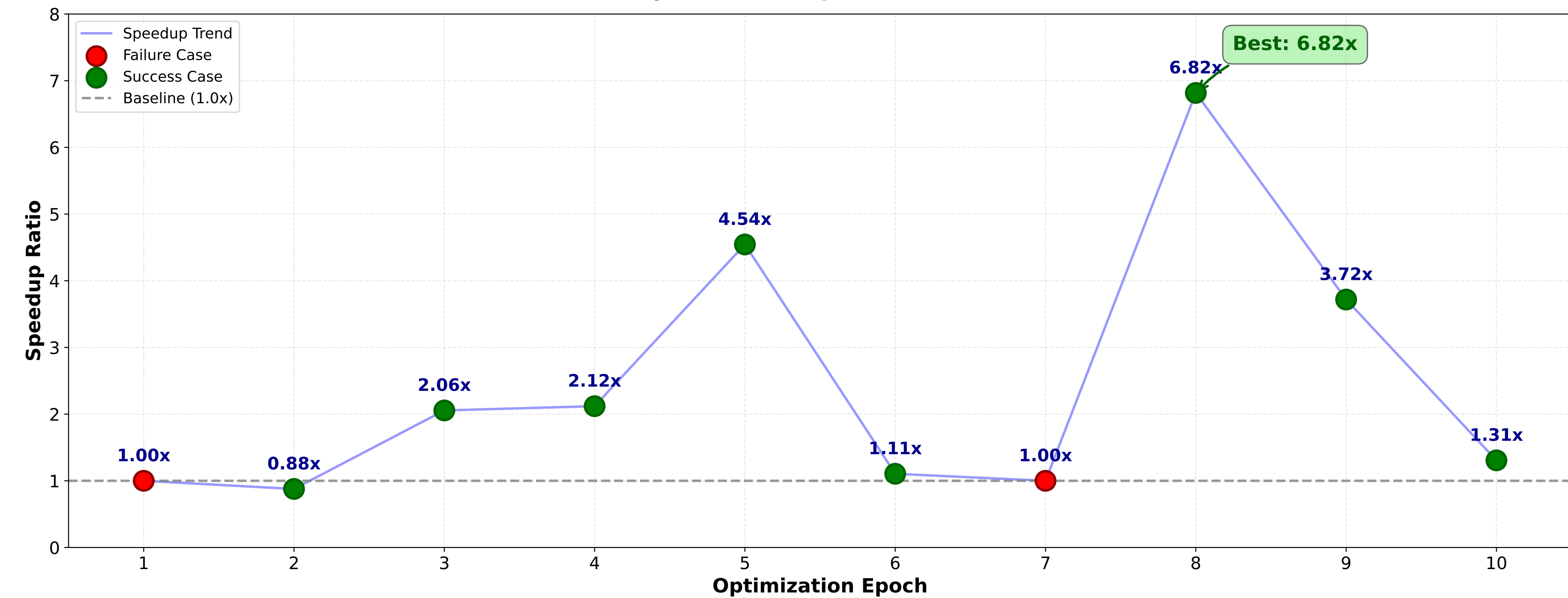
(b) LayerNorm2D Optimization in MNN
