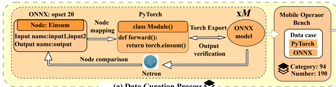
(a) Data Curation Process
