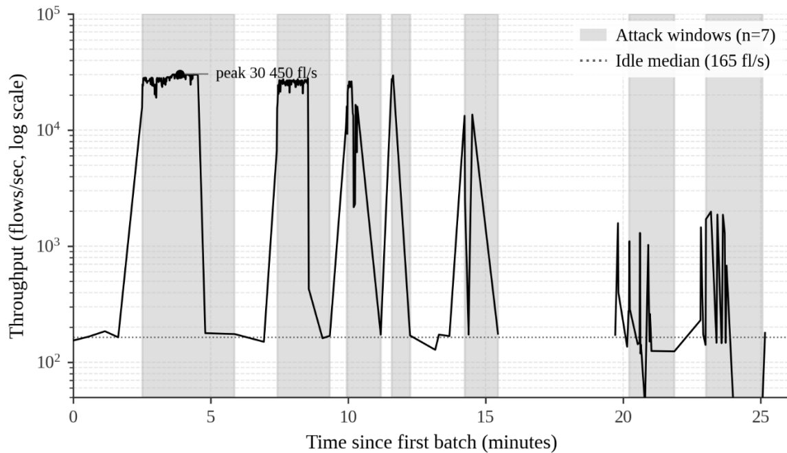
Figure 8 – throughput of the Spark consumer during the live smoke test:
