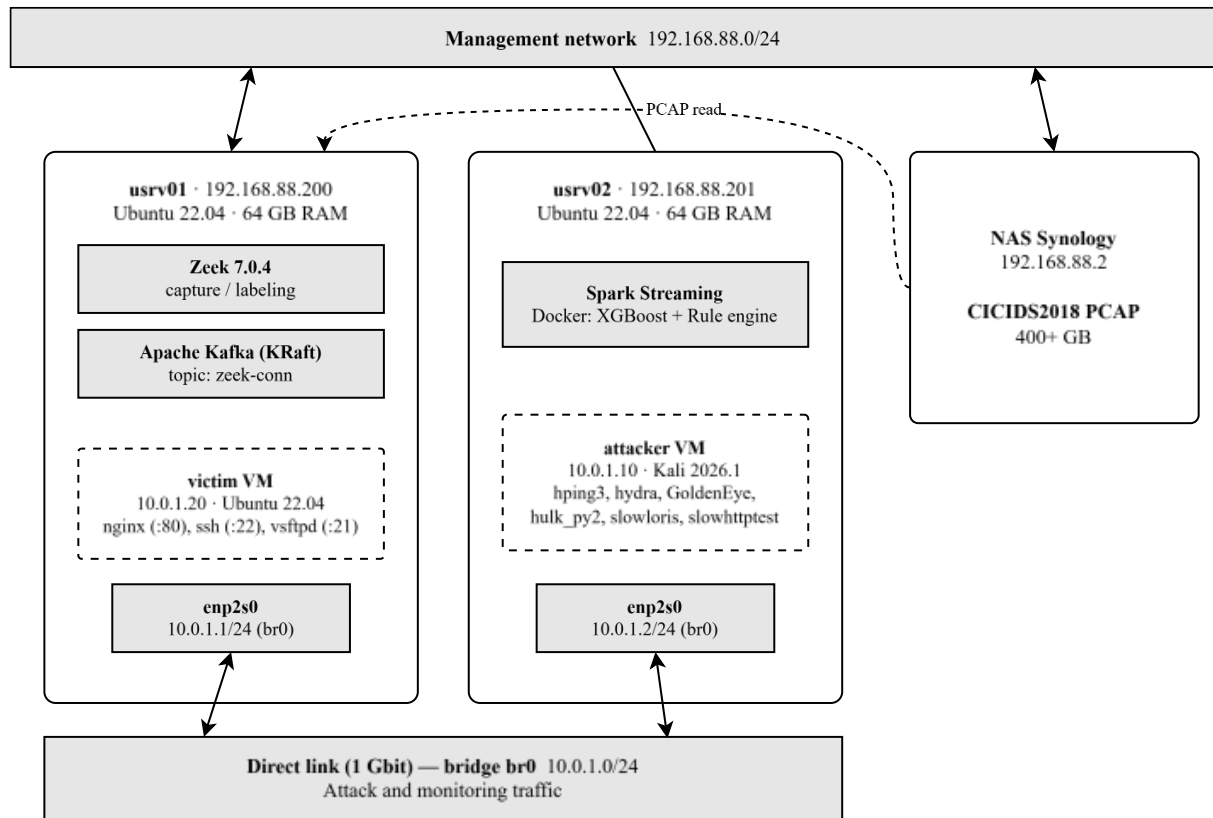
Figure 6 - the lab testbed setup:
