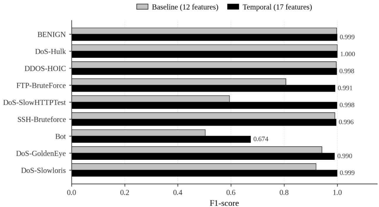
Figure 4 visualizes the per-class F1 improvement:
