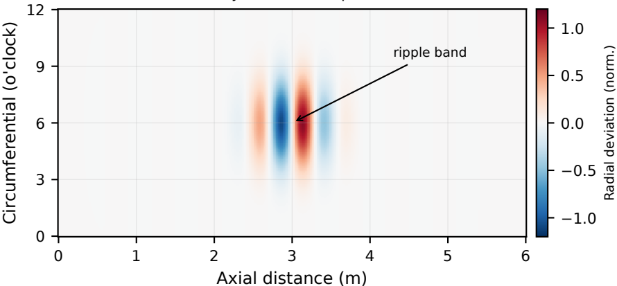
(a) Geometry-ILI radius map (schematic)
