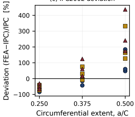
(c) IPC2002 deviation
