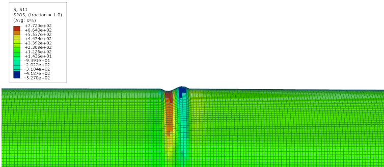
(a) S11 (hoop) contour at ripple, SPOS
