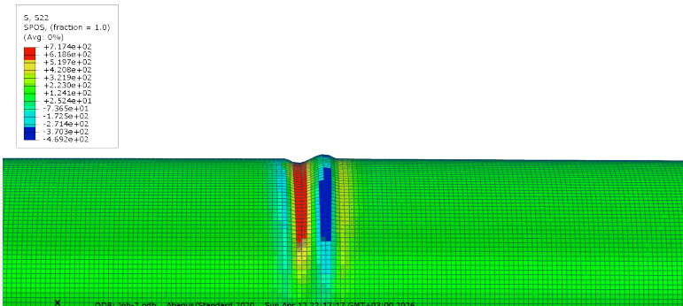
(c) S22 (axial)
