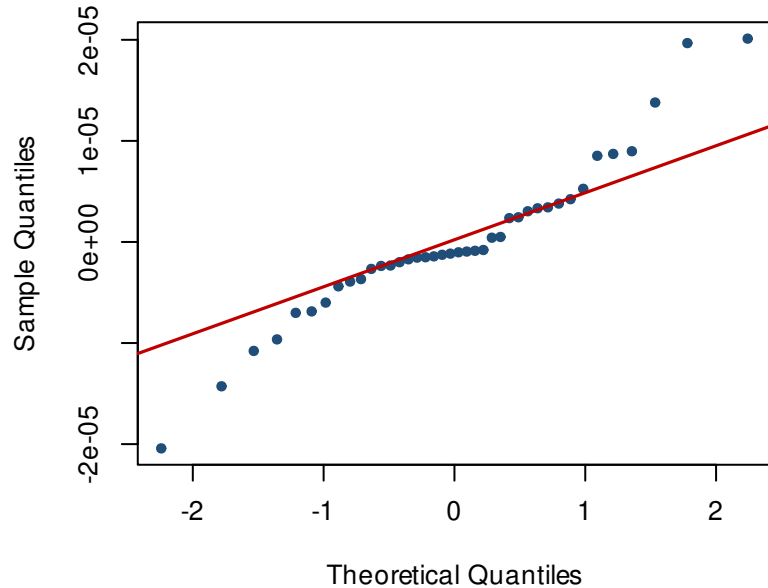
QQ normal
