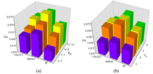
Fig. 12. Hyperparameter sensitivity analyses on three datasets. (a) Patch size P_n . (b) Number of heads V_h .
