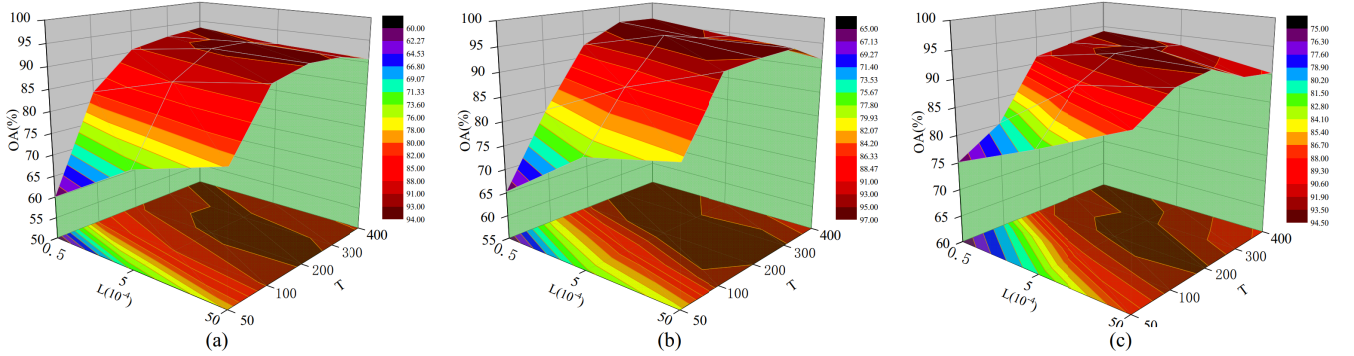
Fig. 11. Hyperparameter sensitivity analysis about the number of epochs T and learning rate L on (a) IP, (b) Salinas, and (c) UH2013.
