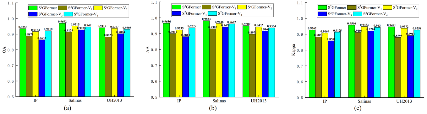
Fig. 13. Ablation experimental results on IP, Salinas, and UH2013. (a) OA. (b) AA. (c) Kappa.
