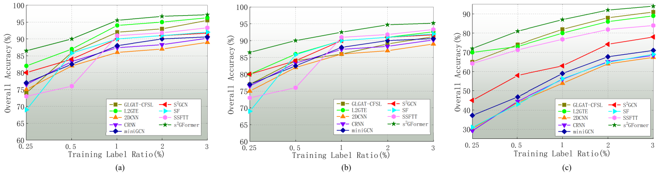
Fig. 10. Overall accuracies (%) of the investigated classifiers with different training label ratios on three datasets. (a) IP. (b) Salinas. (c) UH2013.
