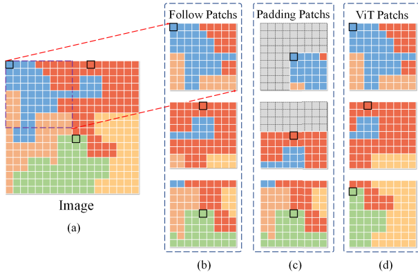
Fig. 2. Illustration of the follow patch mechanism. (a) Input image and (b)–(d) results of the follow patch method, padding patch method, and ViT patch method. Notably, the black-bordered pixels in the figure are the target pixels.
