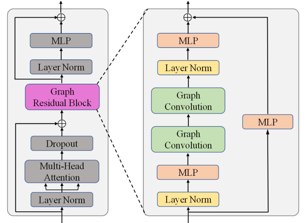
Fig. 4. Illustration of Graphormer Encoder.
