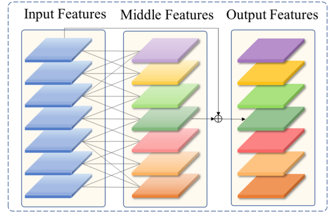
Fig. 3. Illustration of neighborhood convolution.
