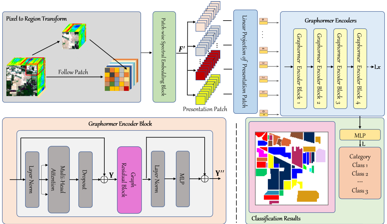
Fig. 1. Illustration of S 2 GFormer for HSI classification. S 2 GFormer mainly consists of three parts, i.e., pixel-to-region transform module, patchwise spectral embedding block, and multilayer Graphormer Encoder module. The pixel-to-region transforms module is proposed to transform the pixels in HSI to locality-preserving regions using follow patch mechanism. The patchwise spectral embedding block is developed to extract the spectral features of the patch. The multilayer Graphormer Encoder module is designed to extract the representative spatial-spectral features from the patch for HSI classification, which is newly designed and essentially different from the Transformer.
