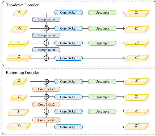
Fig. 3. Illustration of BiDecoder. Interpolation denotes bilinear interpolation and Conv 3 \times 3 , s(\cdot) represents a convolution with kernel size 3 \times 3 and stride is 1 or 2. Upsample indicates that the current feature map will be enlarged to the same size as z_0 .
