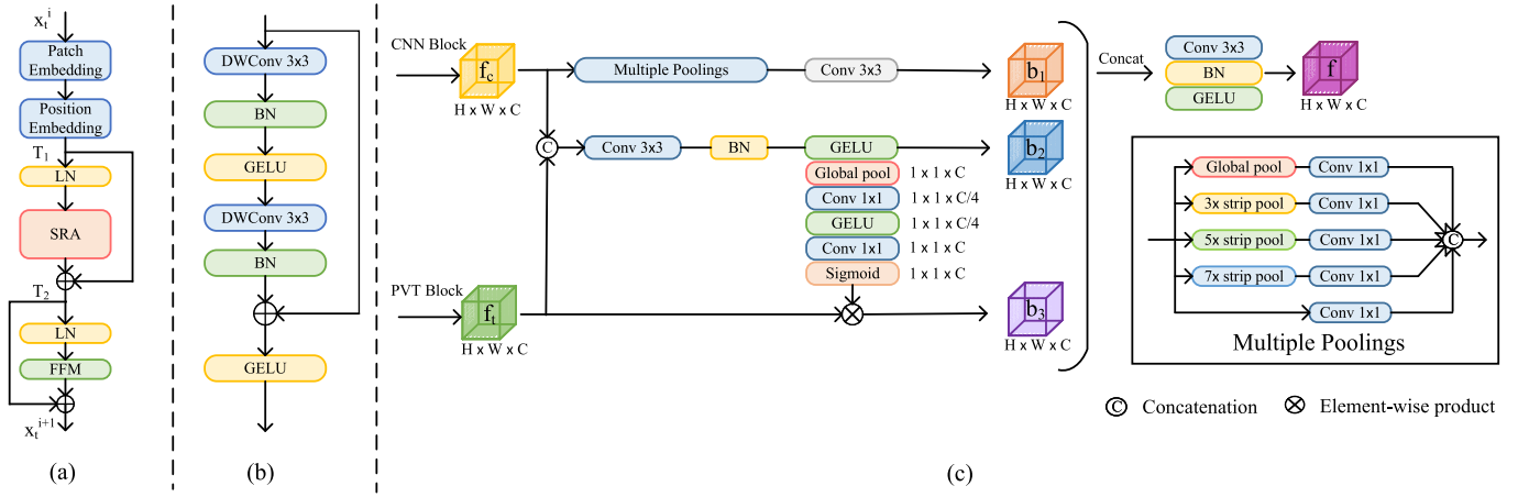
Fig. 2. Illustration of (a) PVT block, (b) CNN block, and (c) FAM. DWConv 3×3 is a depthwise separable convolution with kernel size 3 × 3; BN represents batch normalization; LN is layer normalization; and GELU is the activation function Gaussian error linear unit.
