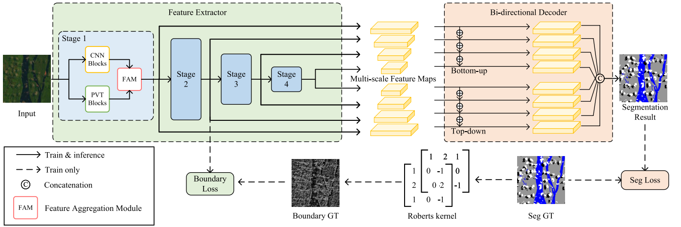
Fig. 1. Overall framework of CTCFNet for semantic segmentation of high-resolution remote sensing images. Multiscale feature maps are composed of the output feature maps of each stage in the feature extractor, and their sizes are 1/4, 1/8, 1/16, and 1/32 of the original image, respectively.
