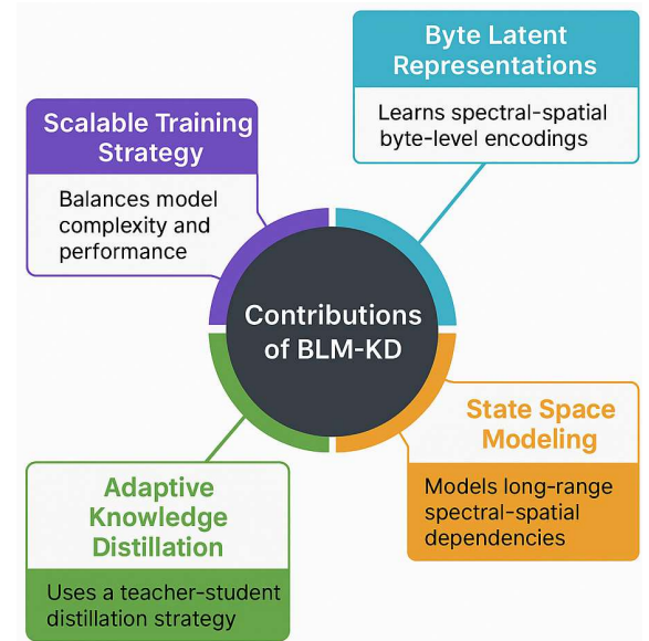
Fig. 1. BLM-KD contribution.
