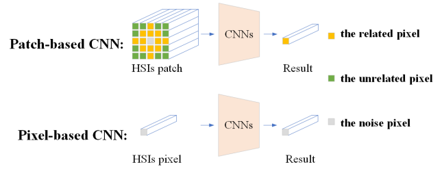
Fig. 1. Patch-based CNN and pixel-based CNN.
