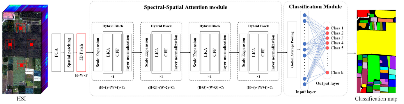
Fig. 4. Overview illustration of the proposed LKSSAN for the HSI classification task. LKSSAN consists of two modules, i.e., SSAM and classification module, and SSAM has two core components: LKA and CFF.
