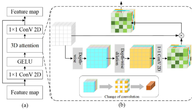
Fig. 6. LKA for spectral-spatial feature learning: (a) detailed structure of LKA in LKSSAN and (b) changes of feature map when using LKA.
