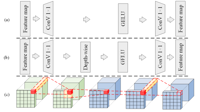
Fig. 7. Structures of feed-forward and convolution feed-forward: (a) feed-forward; (b) convolution feed-forward; and (c) exploded view of convolution feed-forward.
