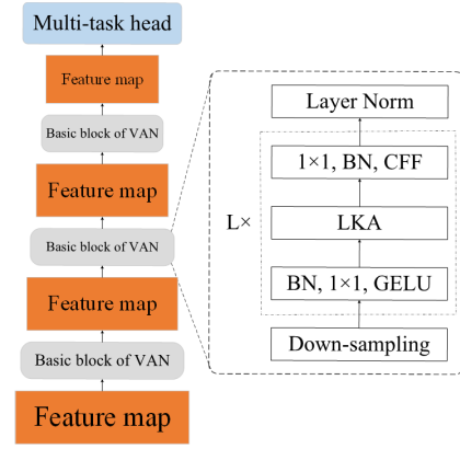
Fig. 3. Original VAN consists of four stages, the scale of the feature map is compressed at each step, and finally uses the multitask head to complete different downstream tasks.
