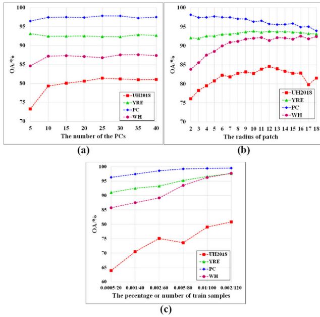
Fig. 12. Effect of: (a) number of PCs; (b) size of patch; and (c) number of training samples on the classification accuracies in the four datasets.
