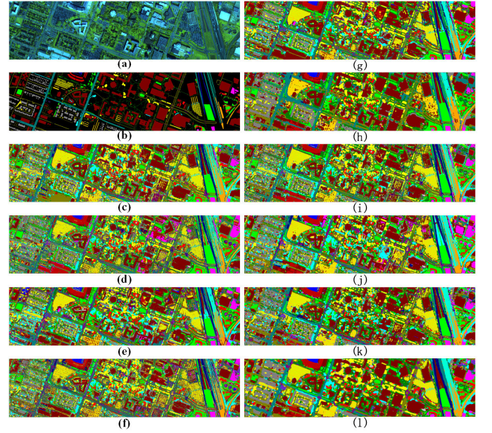
Fig. 13. Classification maps of different methods on UH2018 dataset: (a) false-color image of UH2018; (b) GT; (c) SSRN; (d) MSDN; (e) SSUN; (f) RSSAN; (g) ASSMN; (h) DBDA; (i) A2S2K; (j) SSTN; (k) SSFTT; and (l) LKSSAN.
