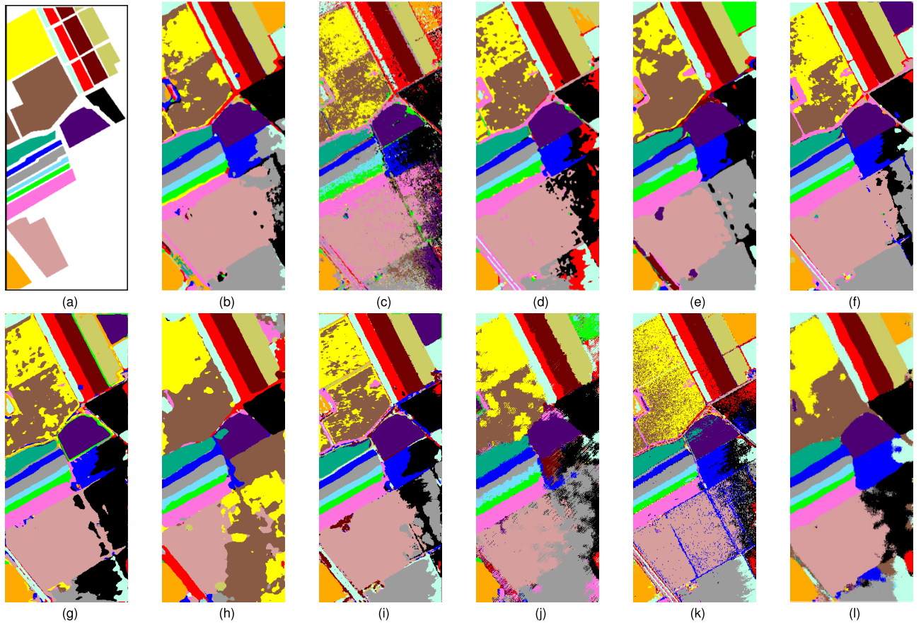
Fig. 9. Classification maps obtained by different methods for Salinas. (a) Ground-truth, (b) 2-D-CNN (90.96%), (c) 3-D-CNN (86.56%), (d) SSRN (88.82%), (e) DPN-HRA (91.08%), (f) S-DMM (91.80%), (g) CMFSL (91.72%), (h) S3Net (94.24%), (i) DCFSL (92.10%), (j) SSFTT (89.17%), (k) miniGCN (81.98%), and (l) DM-MRN (95.12%).
