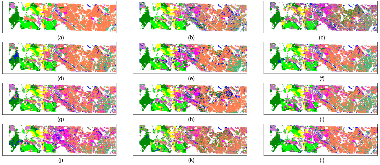
Fig. 11. Classification maps obtained by different methods for Berlin. (a) Ground-truth, (b) 2-D-CNN (57.45%), (c) 3-D-CNN (49.35%), (d) SSRN (53.72%), (e) DPN-HRA (60.60%), (f) S-DMM (55.75%), (g) CMFSL (60.43%), (h) S3Net (53.72%), (i) DCFSL (57.53%), (j) SSFTT (57.91%), (k) miniGCN (49.54%), and (l) DM-MRN (61.64%).
