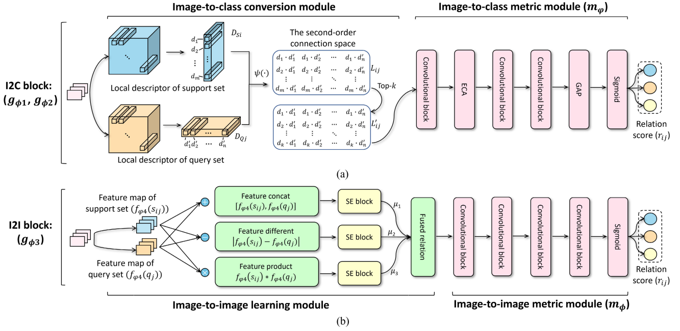
Fig. 2. Architecture of relation module. (a) I2C block. (b) I2I block.
