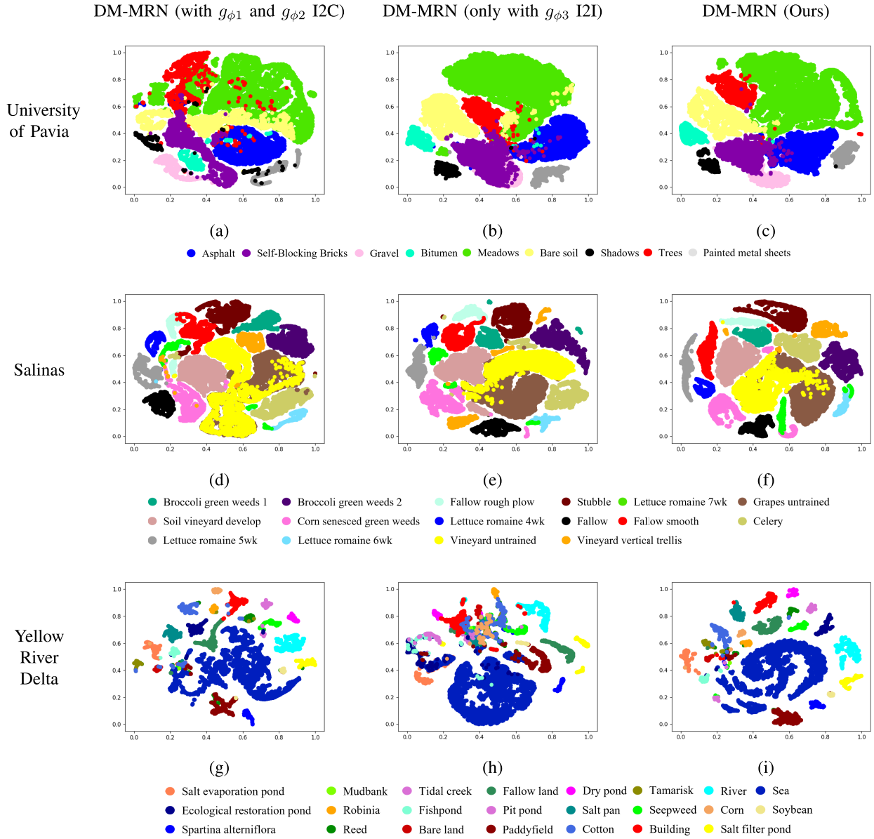
Fig. 13. Visualization of feature separability for different methods. (a) DM-MRN (with g_{\phi_1} and g_{\phi_2} I2C block), (b) DM-MRN (only with g_{\phi_3} I2I block), (c) DM-MRN (Ours) for University of Pavia, (d) DM-MRN (with g_{\phi_1} and g_{\phi_2} I2C block), (e) DM-MRN (only with g_{\phi_3} I2I block), (f) DM-MRN (Ours) for Salinas, (g) DM-MRN (with g_{\phi_1} and g_{\phi_2} I2C block), (h) DM-MRN (only with g_{\phi_3} I2I block), and (i) DM-MRN (Ours) for Yellow River Delta.
