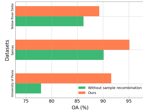
Fig. 6. Ablation analysis of sample recombination of DM-MRN.
