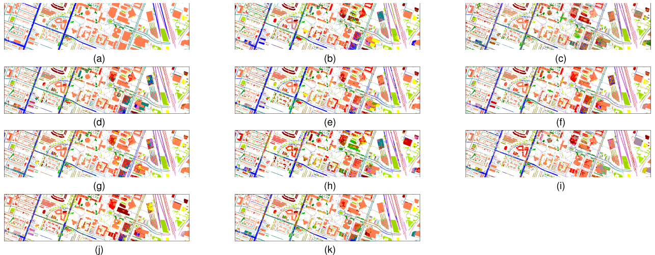
Fig. 12. Classification maps obtained by different methods for Houston2018. (a) Ground-truth, (b) 2-D-CNN (48.04%), (c) 3-D-CNN (36.47%), (d) SSRN (49.27%), (e) DPN-HRA (47.14%), (f) S-DMM (51.34%), (g) CMFSL (50.24%), (h) S3Net (37.38%), (i) SSFTT (49.37%), (j) miniGCN (37.46%), and (k) DM-MRN (55.68%).
