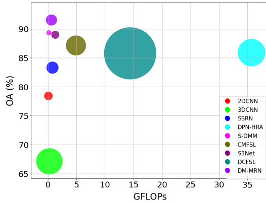
Fig. 14. Comparison of OA, FLOPs, and parameter size of each model in the University of Pavia dataset (ten labeled samples per class).
