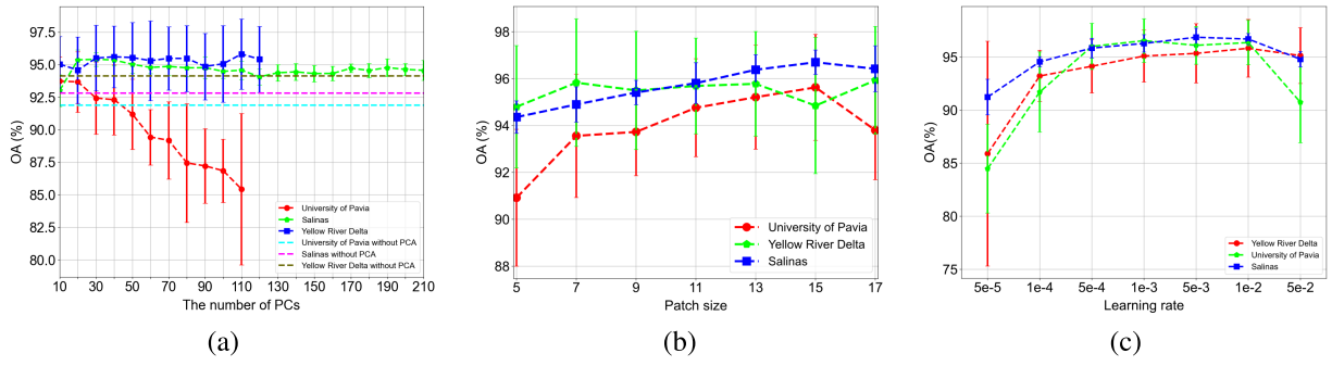
Fig. 4. Evolution of OA as a function of (a) number of PCs, (b) patch size, and (c) learning rate.
