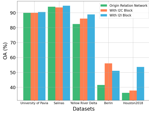
Fig. 7. Ablation analysis of I2C block and I2I block of DM-MRN.
