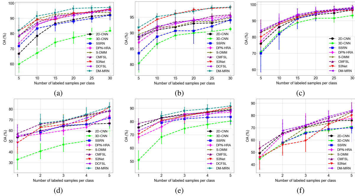
Fig. 5. Evolution of OA as a function of the number of labeled samples per class. (a) 5–30 for the University of Pavia, (b) 5–30 for Salinas, (c) 5–30 for Yellow River Delta, (d) 1–5 for the University of Pavia, (e) 1–5 for Salinas, and (f) 1–5 for Yellow River Delta.
