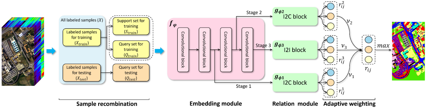
Fig. 1. Flowchart of the proposed DM-MRN for few-shot HSI classification.
