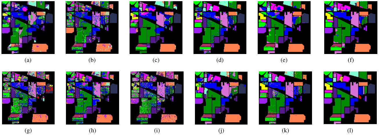
Fig. 7. Classification maps of different methods on the Indian Pines dataset. (a) 3DCNN. (b) ASSMN. (c) DPRN. (d) DSGSF. (e) morphFormer. (f) GraphGST. (g) Cluster-GCN. (h) Funet-C. (i) MiniGCN. (j) GCN. (k) SGDNet. (l) Ground truth.
