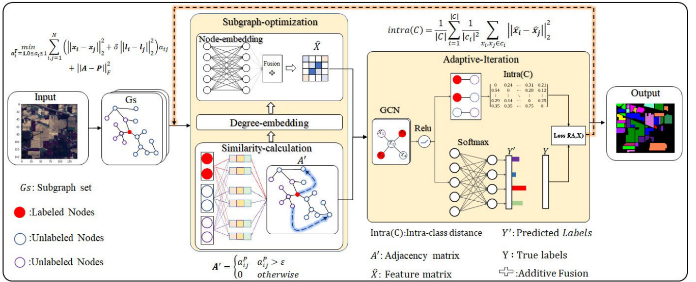
Fig. 1. Algorithmic framework of SGDNet, divided into distinct phases: input, subgraph optimization, adaptive iteration, and output. Within this framework, a dynamic cyclic process occurs that transitions from graph optimization to information aggregation once the criteria for intra-class distance judgment are satisfied.
