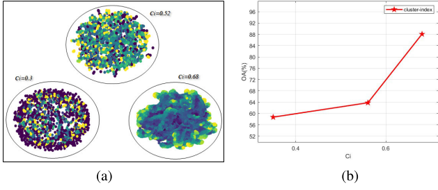
Fig. 2. Indian pines dataset after cutting the molecular map, showing the distribution of each sample point (without edge connections); the color depth represents different categories of samples, C_i represents the clustering coefficient, so as to observe its general topology and spatial structure. (a) Connectivity distribution of three subgraphs. (b) OAs of three subgraphs with two convolution layers.
