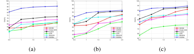
Fig. 11. OAs of different training samples for three HSI datasets. (a) Indian Pines. (b) Houston. (c) PaviaU.
