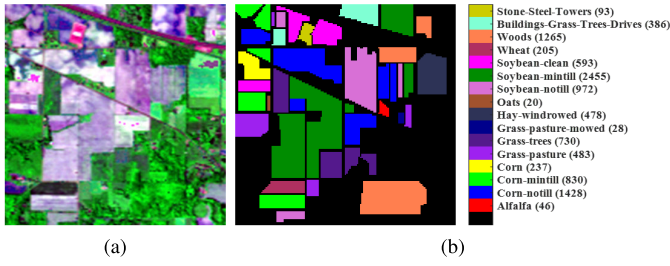
Fig. 4. Indian Pines data. (a) False color image (bands 20, 69, and 178 are red, green, and blue, respectively). (b) Ground-truth image.
