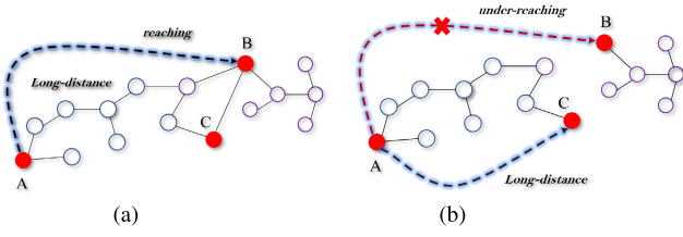
Fig. 3. Changes in sample remote dependence before and after subgraph segmentation, and whether it can be used to display aggregated information. The black dotted line represents reachability, while the red dotted line represents unreachability. (a) Long-range structural dependency of the whole graph. (b) Long-range structural dependency between subgraphs.
