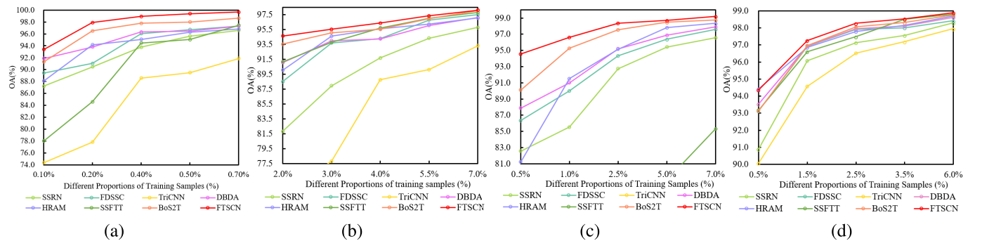
Fig. 12. Classification outcomes obtained by various methods using different proportions of training samples with (a) UP, (b) IP, (c) KSC, and (d) ZY.
