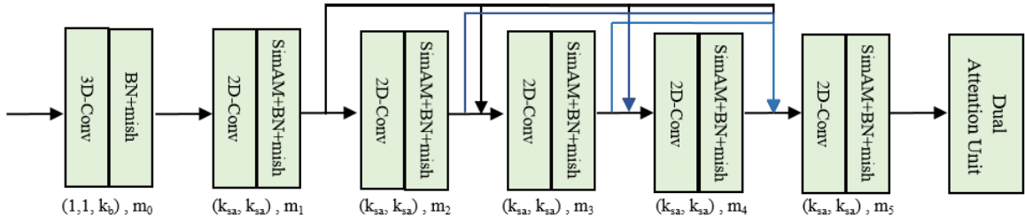
Fig. 3. Architecture of our SimAM-based hierarchical dense network, where 3-D-Conv and 2-D-Conv stand for 3-D and 2-D convolutions, respectively. BN and mish stand for batch normalization and the activation function, separately.
