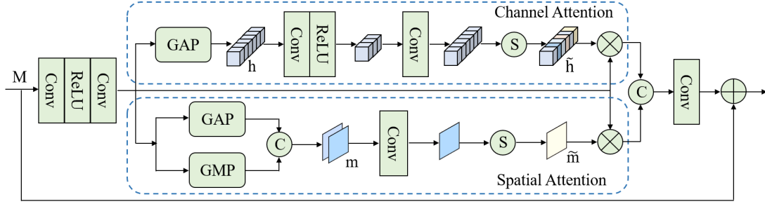
Fig. 4. Structure of the DAU, which includes spatial and channel attention mechanisms. GAP and GMP stand for global average and maximum pooling operations, respectively. \oplus denotes the concatenation operation. \odot denotes the sigmoid function. \oplus and \otimes stand for element-level summation and multiplication, separately.
