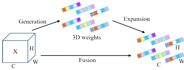
Fig. 1. Graphical illustration of the SimAM attention mechanism, where the complete 3-D weights are for attention.
