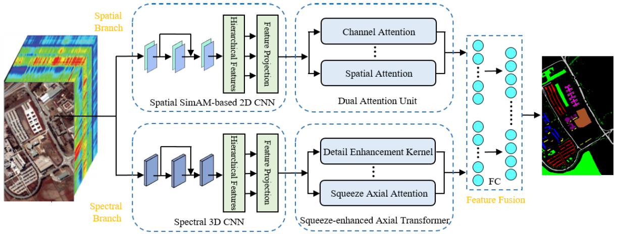
Fig. 2. Flowchart of the proposed FTSCN model that contains a spatial branch, a spectral branch, and a feature fusion branch network. The SimAM-based 2-D-CNN is exploited to build a hierarchical dense network structure to retrieve the hierarchical spatial feature information contained in the original HSI. After that, DAU with spatial and channel attention properties is utilized to improve the capability of the model to acquire spatial characteristics. Besides, the 3-D-CNN is utilized to build a hierarchical dense network structure to extract hierarchical local spectral characteristics from each convolutional layer, and a squeeze-enhanced axial transformer is adopted to boost the spectral signature extraction capacity of the model.
