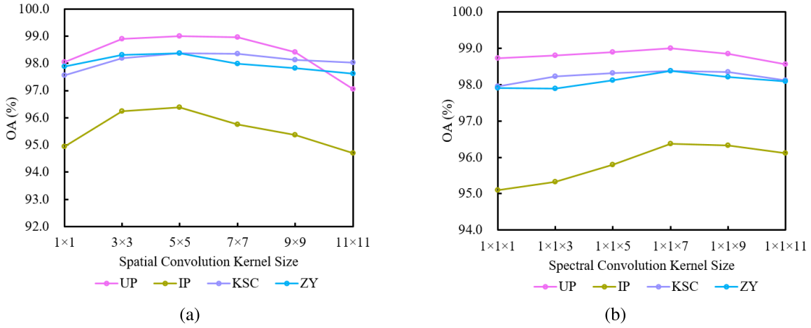
Fig. 7. Variation of FTSCN classification performance with various sizes of (a) spatial and (b) spectral convolutional kernels.
