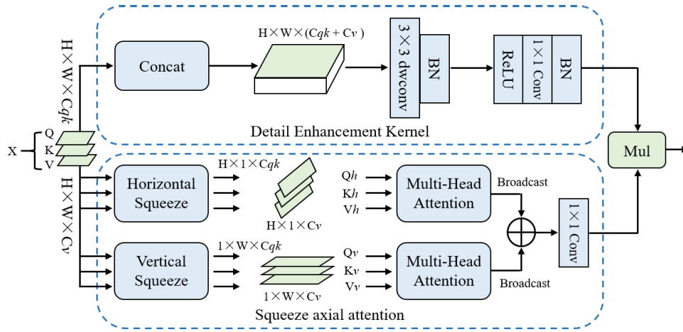
Fig. 5. Architecture of the squeeze-enhanced axial transformer, where \oplus denotes the addition operation and Mul denotes the multiplication operation.
