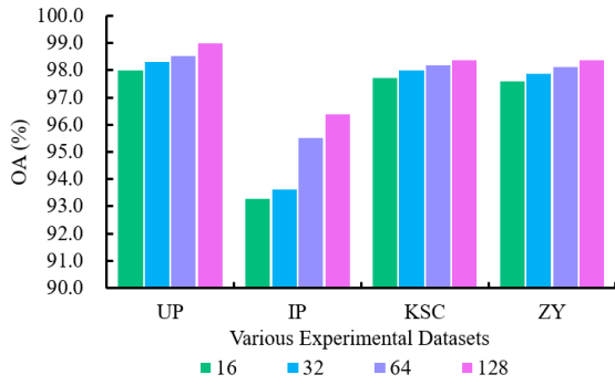
Fig. 6. Variation of classification accuracy for different batch sizes on various datasets.
