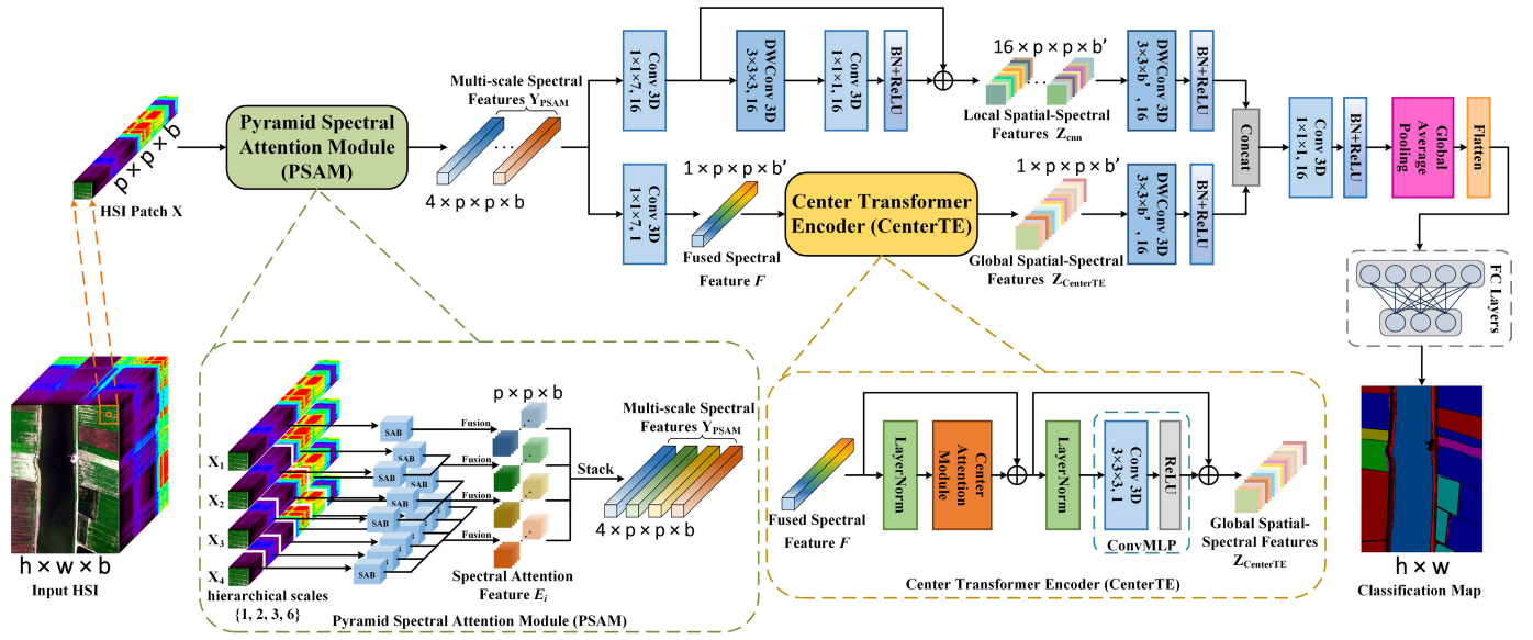
Fig. 2. Overall architecture of CTSSA. BN: batch normalization. ReLU: rectified linear unit activation function.
