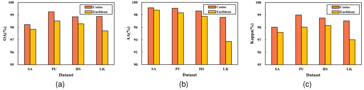
Fig. 11. Ablation study on the choice of similarity function in the CenterTE module. (a) OA. (b) AA. (c) Kappa.
