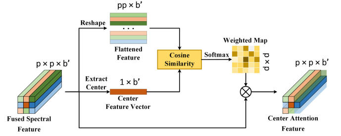
Fig. 4. Overall architecture of the proposed CAM module.
