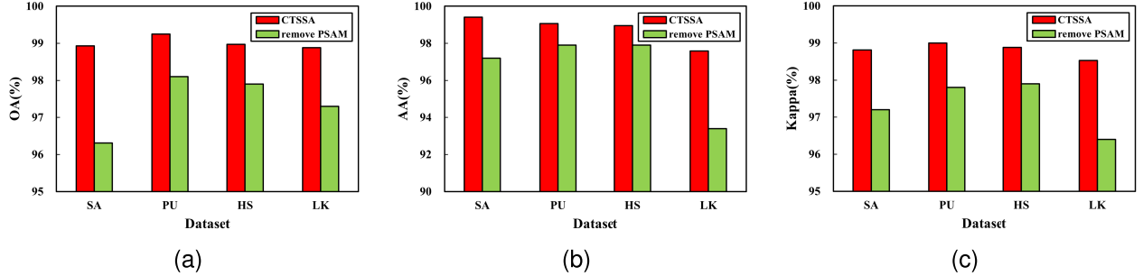
Fig. 10. Ablation study on the accuracy metrics for the PSAM module. (a) OA. (b) AA. (c) Kappa.
