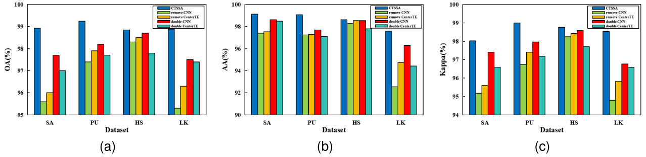
Fig. 12. Ablation study on the accuracy metrics for the dual branch. (a) OA. (b) AA. (c) Kappa.
