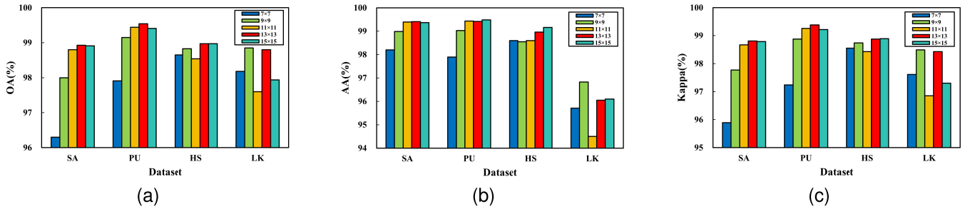
Fig. 13. Accuracy metrics of CTSSA with different patch sizes on four datasets. (a) OA. (b) AA. (c) Kappa.
