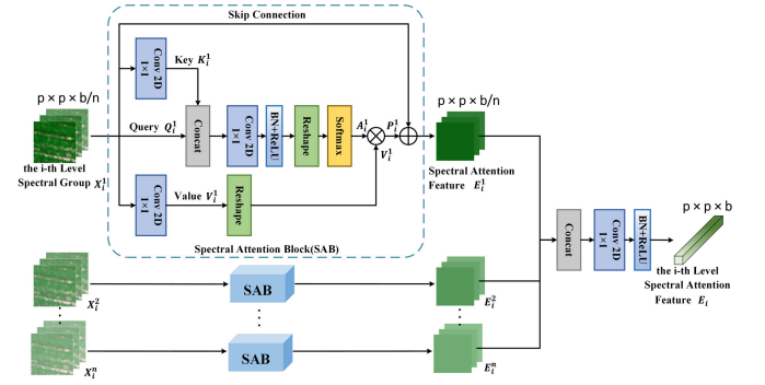
Fig. 3. Architecture of the proposed SAB module.
