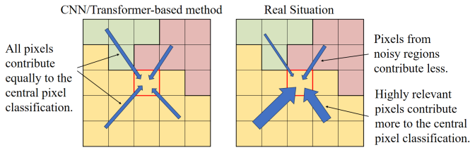
Fig. 1. Comparison of pixel contribution assumptions within a patch (taking a 5 \times 5 patch as an example, with the central pixel indicated by the red box): CNN/transformer-based methods versus the real situation.
