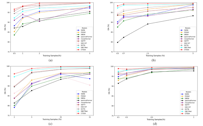
Fig. 5. Quantitative results with different numbers of training samples per class. (a) SA. (b) PU. (c) HS. (d) LK.
