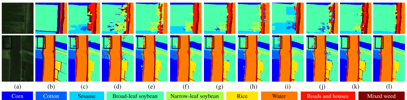
Fig. 9. Classification maps of different methods on the LK dataset. (a) False-color image. (b) Ground truth. (c) AMGCFN. (d) GSC-ViT. (e) MASSFormer. (f) S^2 GFormer. (g) PSFormer. (h) DBCT. (i) GiGCN. (j) NESSGGCN. (k) SSEFN. (l) SPGFormer.
