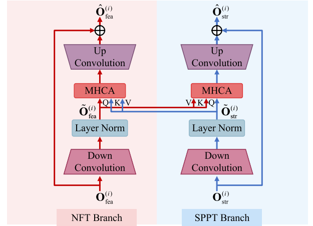
Fig. 4. Structure diagram of BCAM. The MHCA is employed to enable information interaction between the two branches.
