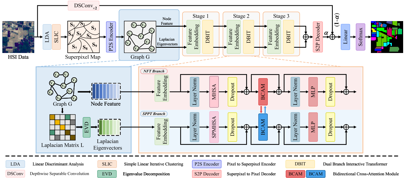
Fig. 1. Overall structure of the SPGFormer framework. SPGFormer primarily consists of three components: the graph construction module, the DBIT module, and the BCAM. The graph construction module segments the original HSI into superpixels and builds a corresponding graph structure. The DBIT module captures rich spatial-spectral information. The BCAM facilitates information exchange between the two branches of the DBIT module, enabling a more comprehensive feature representation.
