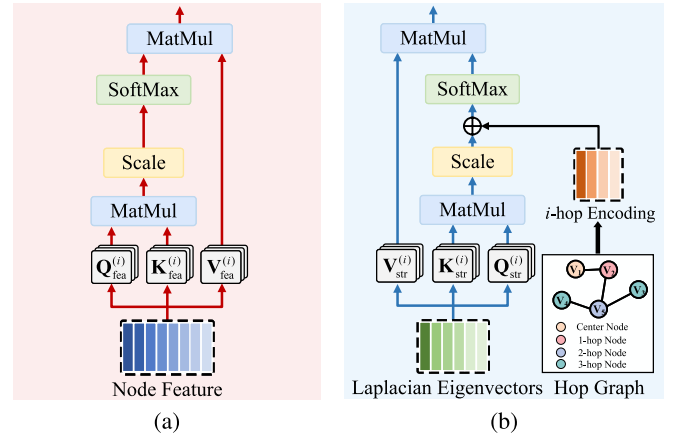
Fig. 3. Structure diagram of (a) MHSA mechanism and (b) SPMHSA mechanism.
