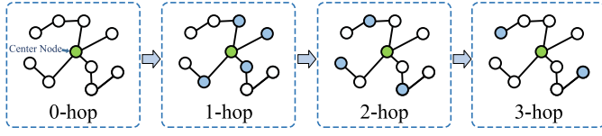
Fig. 2. Schematic of the hop graph structure. The green node indicates the center node, and the blue nodes are its k -hop neighbors.
