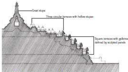
10.00 Partial section showing the three levels of Borobudur
