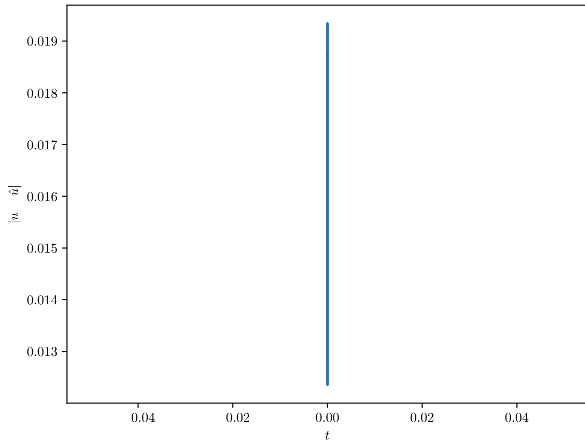
Prediction error
