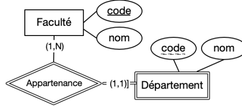
Figure 3. Exemples notation Chen (Elmasri-Navathe)
