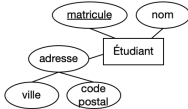
Figure 3. Exemples notation Chen (Elmasri-Navathe)
