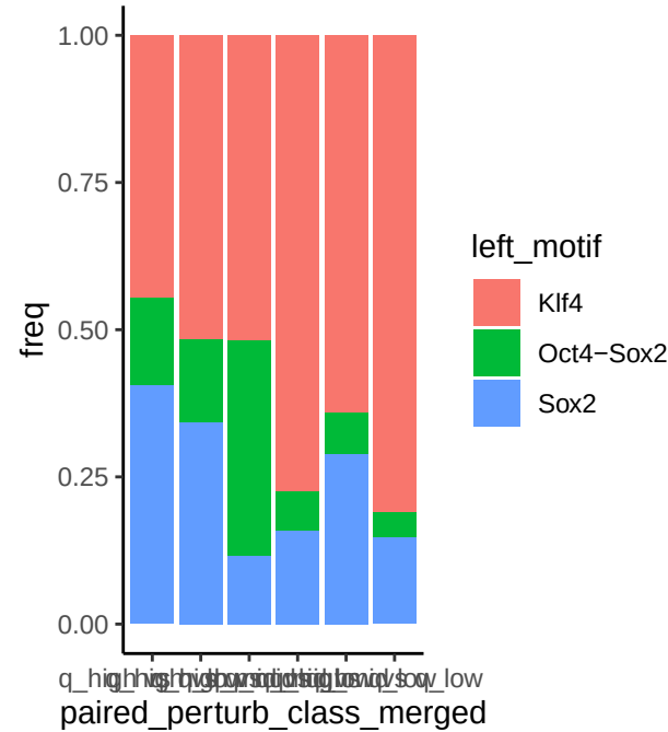
motifA identities
