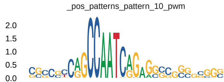
fold1_atac_wt
