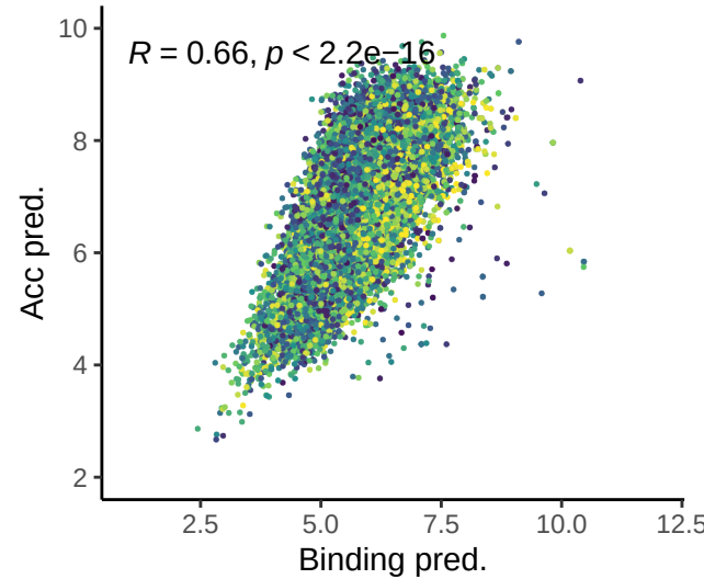
Oct4-Sox2
