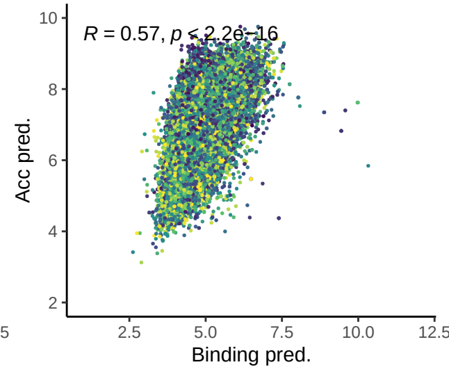
Sox2
