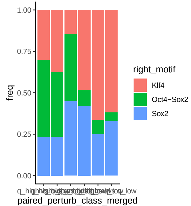
motifB identities
