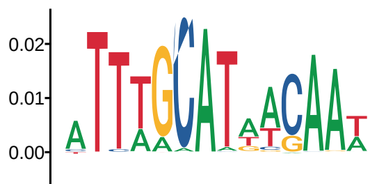
Oct4-Sox2_3h
